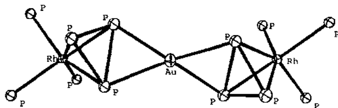
Fig. 17. Inner skeleton of the [\text{Au}\{(\text{triphos})\text{Rh}(\text{P}_3)\}_2]^+ cation ( 15 ).
