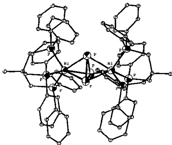
Fig. 2. A view of the [(\text{triphos})\text{Ni}(\text{P}_3)\text{Ni}(\text{triphos})]^{2+} cation, representative of compounds of group 2.
