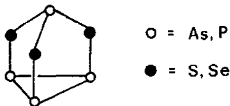
Fig. 3. The atomic arrangement in a \text{E}_4\text{X}_3 molecule.
