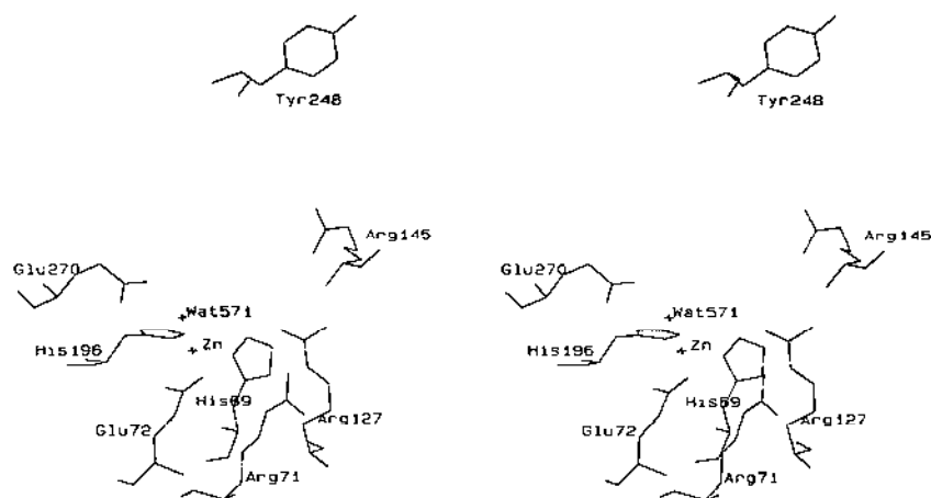
Fig. 2. Stereoview of the native CPA active site cavity. Coordinates are from ref. 13.
