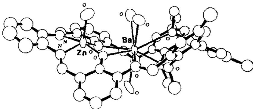
Fig. 75. Structure of \text{ZnBa(100)(CF}_3\text{SO}_3)_2 \cdot 3\text{dmf} (only the coordinated oxygen atoms of the three dimethylformamide molecules and of the coordinated anion are shown for clarity).
