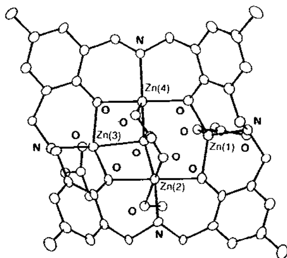
Fig. 114. The structure of \text{Zn}_4(\mathbf{131})(\text{OH})(\text{CH}_3\text{COO})_3 .
