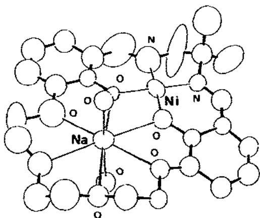
Fig. 74. View of \text{NaNi(98)(picrate)} (only the coordinated oxygen atoms of the two picrate anions are shown for clarity).
