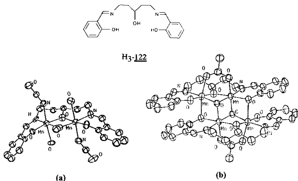
Fig. 97. Structures of (a) [\text{Mn}_2(\text{122})(\text{CH}_3\text{O})(\text{NCO})_2(\text{H}_2\text{O})_2] and (b) [\text{Mn}_4(\text{122})_2(\text{O})_2(\text{CH}_3\text{COO})_2] .
