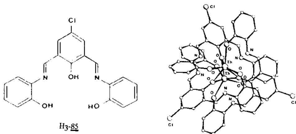
Fig. 66. Structure of [\text{Th}_2(\text{85})_3]_2^{2-} .
