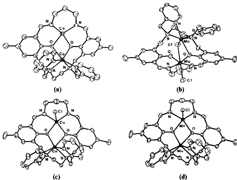
Fig. 76. Structures of (a) [\text{Co}_2(\text{B})](\text{PF}_6)_2 , (b) [\text{Mn}_2(\text{B})(\mu\text{-Cl})(\text{Cl})]\text{PF}_6 , (c) [\text{Co}_2(\text{B})(\text{Cl})]\text{PF}_6 and (d) [\text{Mn}_2(\text{B})(\text{Cl})]\text{PF}_6 ( \text{H}_2\text{-B} is the macrocycle reported in Scheme 34).
