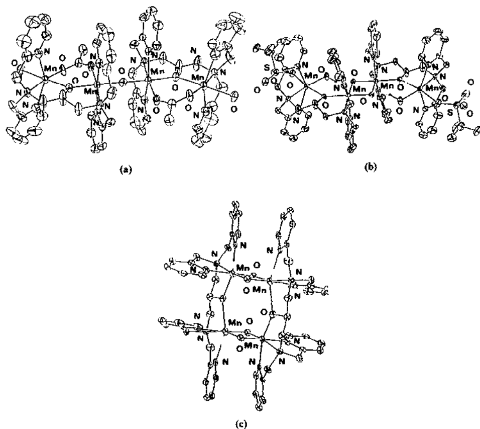
Fig. 100. Structures of (a) \{[\text{Mn}_2(\mathbf{123})(\text{CH}_3\text{COO})(\text{H}_2\text{O})_2]\text{O}\}^{4+} , (b) [\text{Mn}_4\text{O}_2(\mathbf{123})(\text{H}_2\text{O})_2(\text{CF}_3\text{SO}_3)_2]^{3-} and (c) [(\text{Mn}_2\text{O}_2)_2(\mathbf{123})_2]^{4+} .
