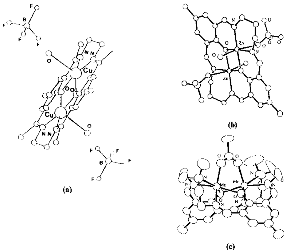
Fig. 58. Structures of (a) [\text{Cu}_2(75)(\text{H}_2\text{O})_2](\text{BF}_4)_2 , (b) [\text{Zn}_2(75')(\text{H}_2\text{O})_2(\text{ClO}_4)_2] and (c) [\text{Mn}_2(75'')(\text{CH}_3\text{COO})_4]^+ .
