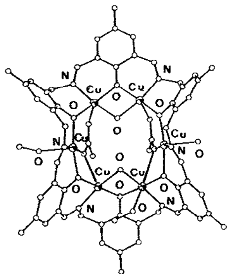
Fig. 115. View of the [\text{Cu}_6(\mathbf{132})(\text{CH}_3\text{COO})_2(\text{OH})_2(\text{MeOH})_2(\text{H}_2\text{O})_2]^{2+} cation.
