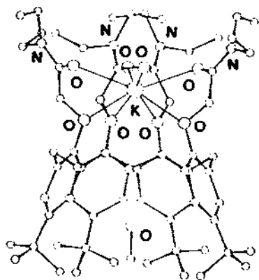
Fig. 6. Structure of K(10) \cdot SCN \cdot MeOH .
