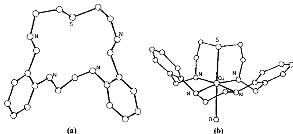
Fig. 42. Structures of (a) 62d and (b) [Cu(62d)(H_2O)]^{2+} .
