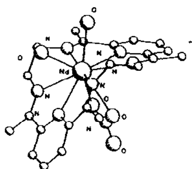
Fig. 50. Structure of [\text{Nd}(\text{NO}_3)_2(\mathbf{38})(\text{H}_2\text{O})_2]^{2+} .
