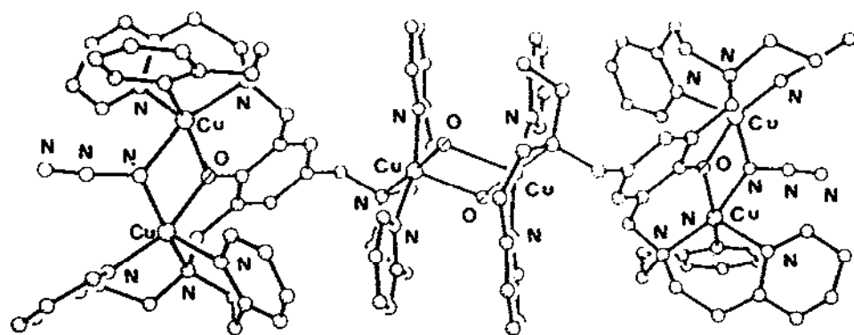
Fig. 78. Perspective view of \{[\text{Cu}_3(\text{105})(\text{N}_3)(\text{OH})]\}_2^{6+} .
