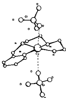
Fig. 34. Structure of [\text{Cu}(\mathbf{52})(\text{ClO}_4)_2] .
