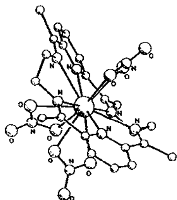
Fig. 48. Structure of [\text{La}(\mathbf{38})(\text{NO}_3)_3] .
