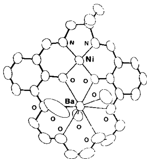
Fig. 73. Structure of \text{NiBa(98)(CF}_3\text{SO}_3)_2 \cdot \text{H}_2\text{O} .
