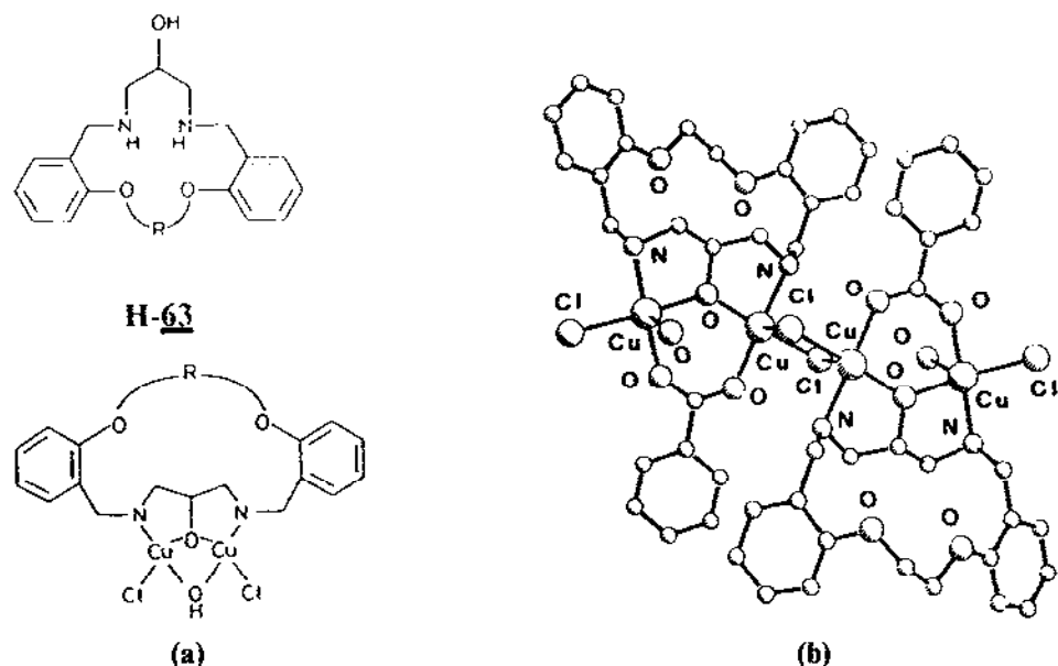
Fig. 45. (a) The proposed structure of the homodinuclear complex \text{Cu}_2(63)(\text{Cl})_2(\text{OH}) . (b) The molecular structure of the tetranuclear complex [\text{Cu}_4(63)(\mu\text{-O}_2\text{CPh})(\text{H}_2\text{O})(\text{Cl})_2] \cdot 2\text{PhCH}_2\text{OH} .
