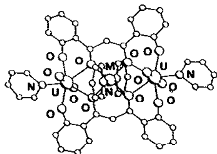
Fig. 88. Perspective view of [(\text{UO}_2)_2\text{M}(\underline{\text{112}})_2(\text{py})_4] \cdot 2\text{py} ( \text{M} \equiv \text{Co}, \text{Ni} )
