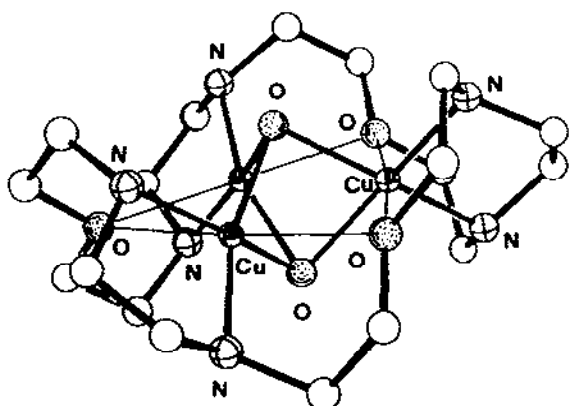
Fig. 132. Structure of [\text{Cu}_3(\mathbf{159})(\text{OH})_2]^{4+} .
