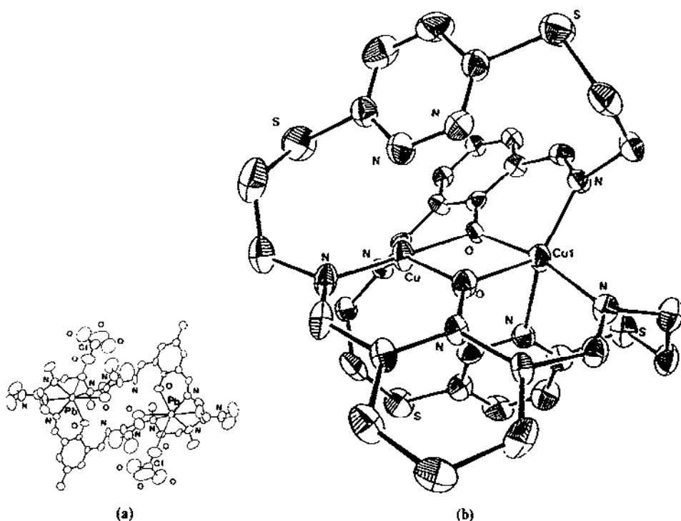
Fig. 118. Structures of (a) [\text{Pb}_2-(\text{H}_2-86'')(\text{dmf})_4(\text{ClO}_4)_2]^{2+} and (b) [\text{Cu}_2(86'')]^{2+} .
