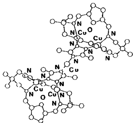
Fig. 122. Structure of [\text{Cu}_5(\text{136})_2(\text{dmt})_2]^{3+} .
