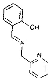
H-115
