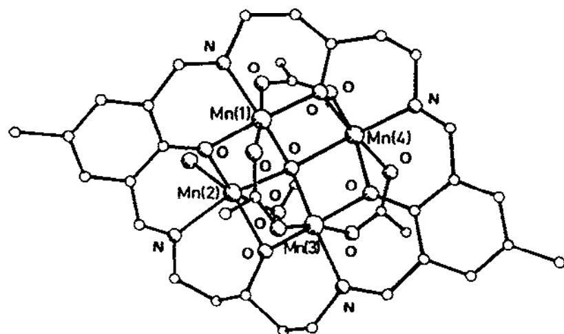
Fig. 111. Structure of [\text{Mn}^{\text{II}}\text{Mn}^{\text{II}}(128)(\text{O})(\text{CH}_3\text{COO})_3(\text{Cl})(\text{MeOH})] .
