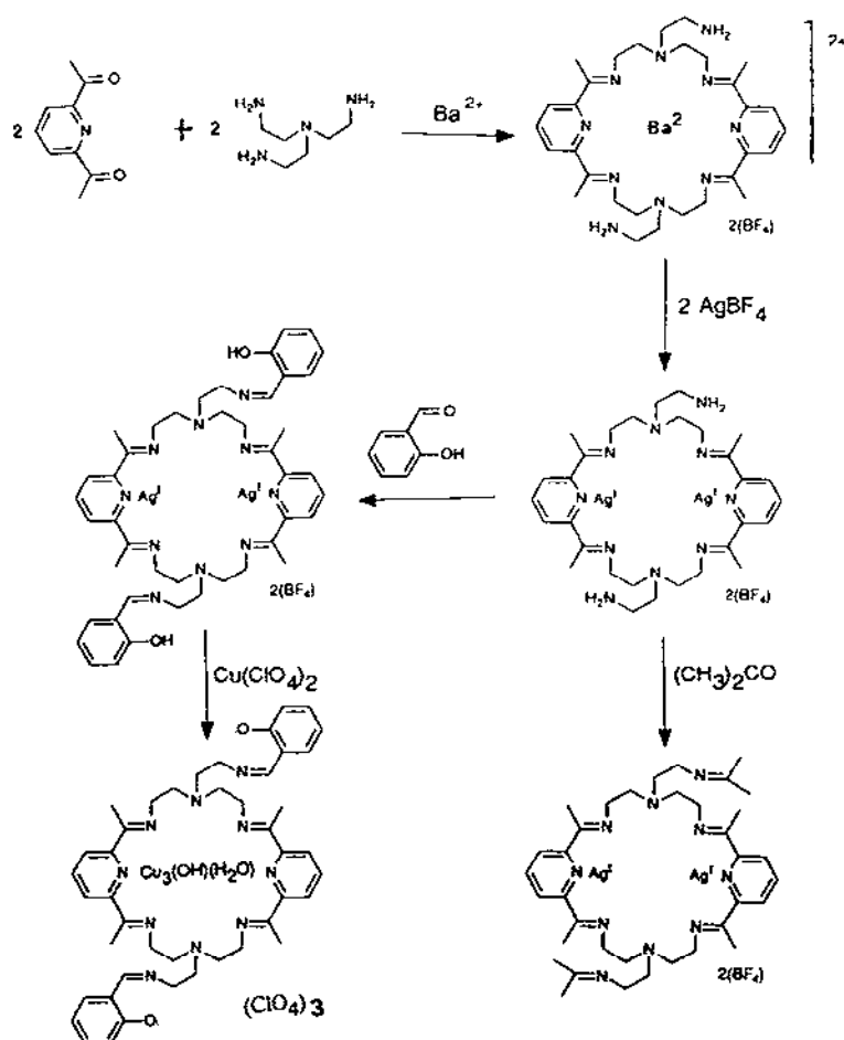
Scheme 36. Reaction pathway for the formation of mononuclear, homodinuclear and homotrimeric complexes.
