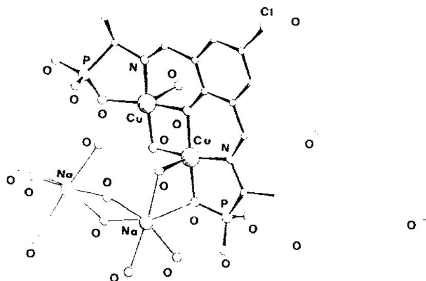
Fig. 64. Structure of [\text{Na}_2\text{Cu}_2(\mathbf{83})(\text{OH})] \cdot 11\text{H}_2\text{O} .
