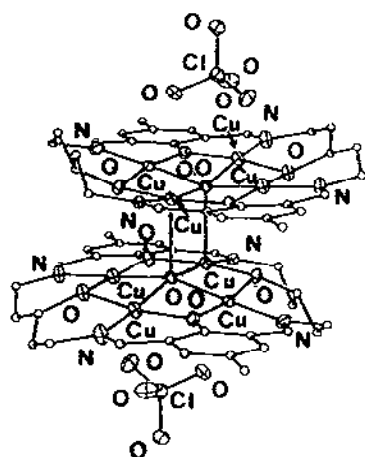
Fig. 116. Perspective view of [\text{Cu}_4(\mathbf{128})(\mu_5\text{-O})(\text{ClO}_4)_2]_2^+ .
