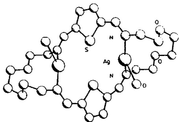
Fig. 12. Structure of [\text{Ag}(\mathbf{27}')(\text{H}_2\text{O})]^{2-} .
