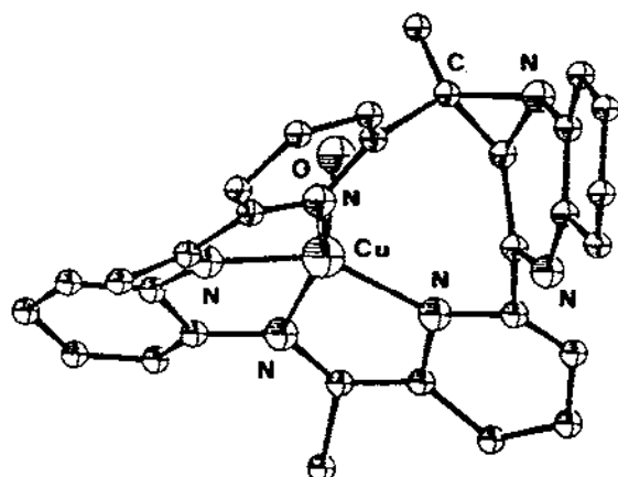
Fig. 16. Structure of [\text{Cu}(\mathbf{35})(\text{H}_2\text{O})]^{2+} .
