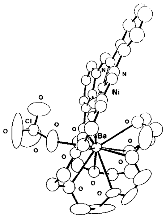
Fig. 72. Structure of \text{NiBa(97)(ClO}_4)_2 \cdot \text{MeOH} .
