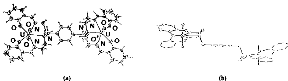
Fig. 124. (a) The molecular structure and (b) the three step conformation of the complex (\text{UO}_2)_2(\mathbf{143}) .
