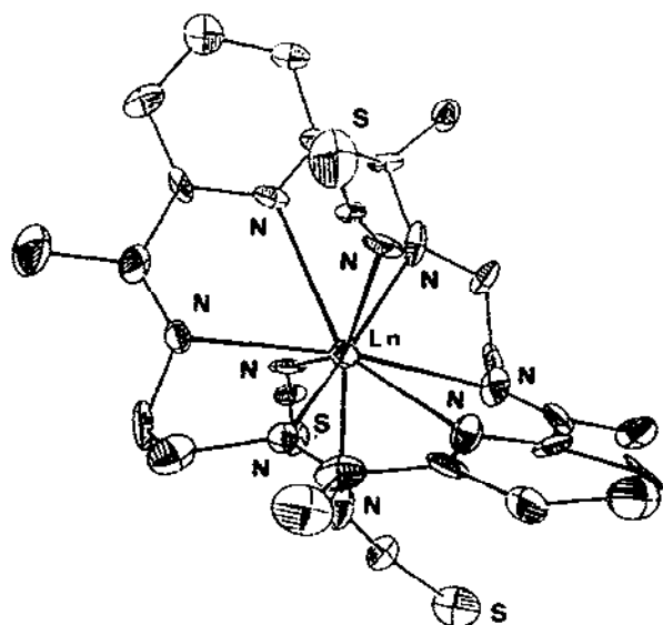
Fig. 54. Structure of [\text{Ln}(\mathbf{38})(\text{NCS})_3] ( \text{Ln} = \text{Y(III)}, \text{Eu(III)} ).
