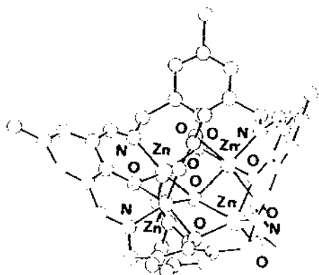
Fig. 113. Structure of \text{Zn}_4(\mathbf{130})(\mu_4\text{-OH})(\text{CH}_3\text{CO}_2)_3 .
