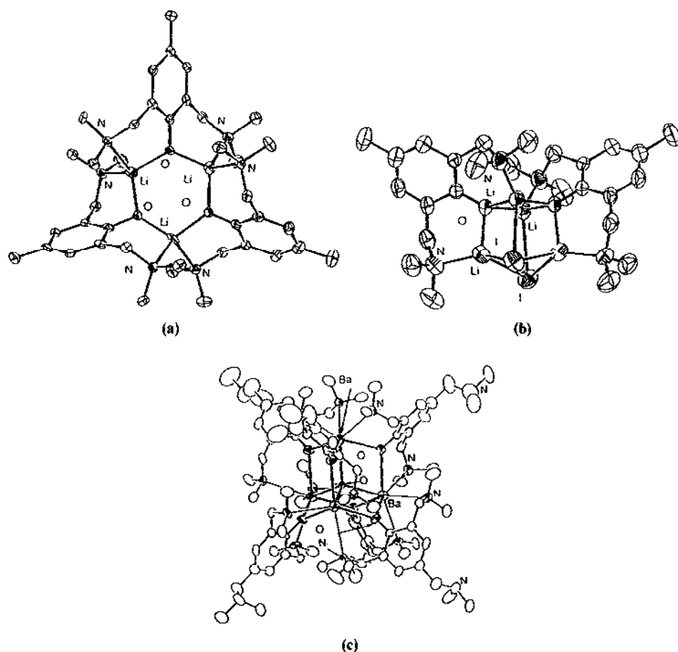
Fig. 101. Structures of (a) [\text{Li}(\mathbf{123'})]_3 , (b) [\text{Li}_4(\mathbf{123'})_2(\text{I})_2] and (c) [\text{Ba}_4(\mathbf{123'})(\mu_4\text{-O})_6] \cdot 3 \text{ toluene} .
