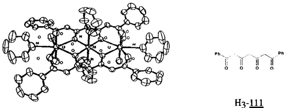
Fig. 87. Structure of [(\text{UO}_2)_2\text{M}(\text{H-111})_2(\text{py})_4] ( \text{M} = \text{Zn}^{2+}, \text{Cu}^{2+}, \text{Ni}^{2+}, \text{Co}^{2+}, \text{Fe}^{2+}, \text{Mn}^{2+} ).
