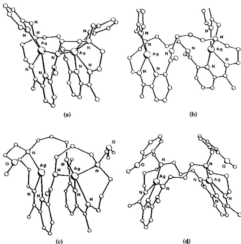
Fig. 37. Structures of (a) [\text{Ag}_2(54)]^{2+} , (b) [\text{Ag}_2(55)]^{2+} , (c) [\text{Ag}_2(56)]^{2+} and (d) [\text{Ag}_2(57)]^{2+} .
