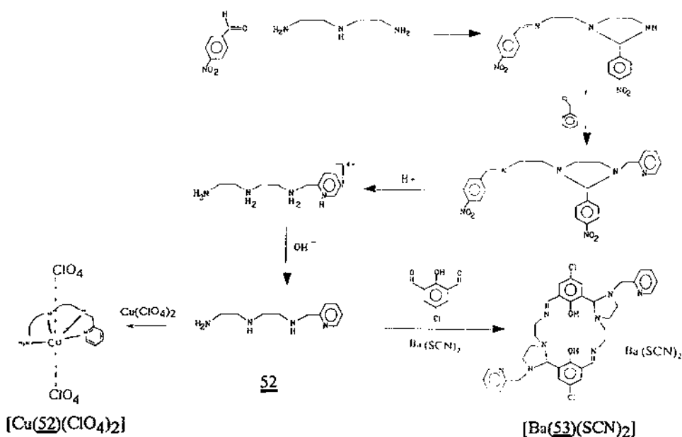
Scheme 20. Preparation of the polyamine 52 and related [\text{Cu}(\mathbf{52})(\text{ClO}_4)_2] and [\text{Ba}(\mathbf{53})(\text{SCN})_2] complexes.
