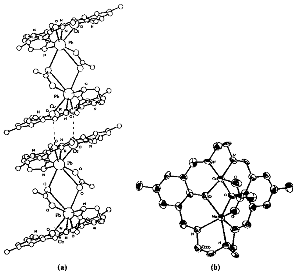
Fig. 84. Structures of (a) [CuPb(109')(CH_3COO)]^+ and (b) [CuMn(109')(CH_3COO)]^+ .
