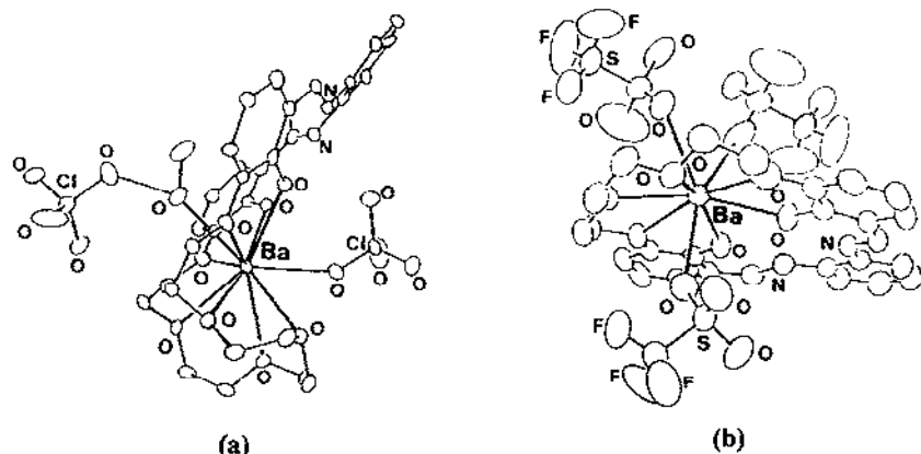
Fig. 25. Structures of (a) \text{Ba}(\mathbf{40})(\text{ClO}_4)_2 \cdot \text{MeOH} and (b) \text{Ba}(\mathbf{41})(\text{CF}_3\text{SO}_3)_2 .
