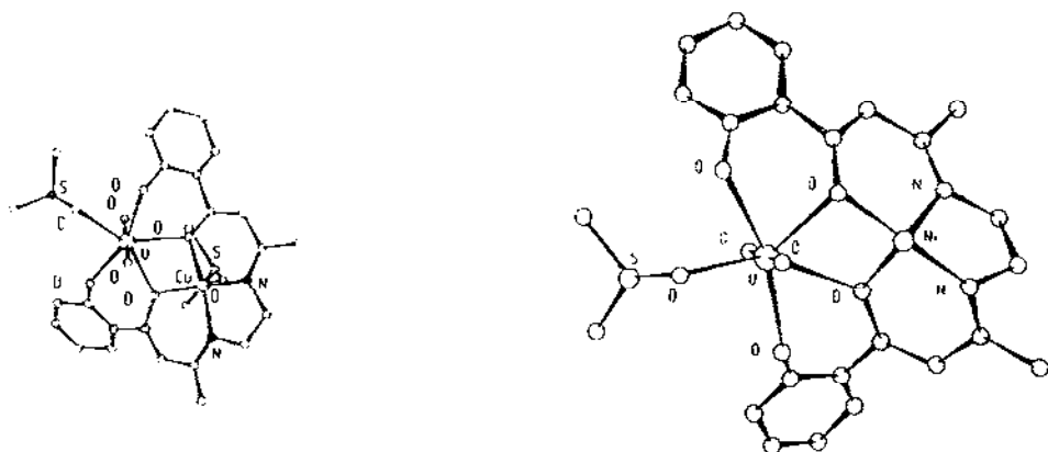
Fig. 62. Structures of (a) [\text{CuUO}_2(79)(\text{dmsO})_2] and (b) [\text{NiUO}_2(79)(\text{dmsO})] .
