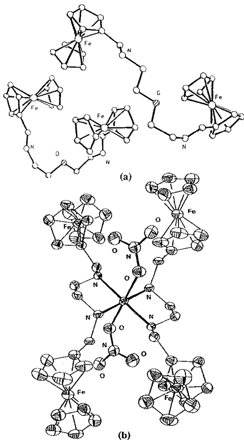
Fig. 125. Structures of (a) diferrocenyl Schiff base reported in Scheme 52 ( R = -(CH_2)_2O(CH_2)_2- ) and (b) bis( N,N' -ethylene bis[ferrocenylmethyl]amine)copper(II) dinitrate.
