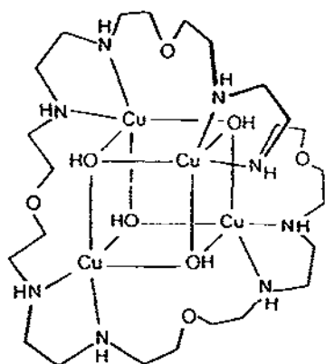
Fig. 133. Probable structure of [\text{Cu}_4(\mathbf{160})(\text{OH})_4]^{4+} .
