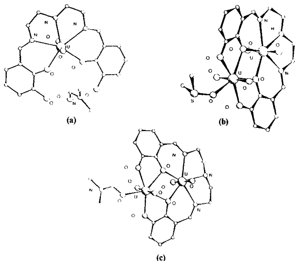
Fig. 71. Structures of (a) \text{UO}_2(\text{H}_2\text{-94}) , (b) (\text{UO}_2)_2(\text{94})(\text{dmsO}) and (c) (\text{UO}_2)_2(\text{94})(\text{dmf}) .
