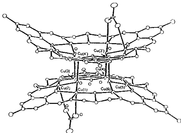
Fig. 109. The structure of [\text{Cu}_6(127e)(\mu_2\text{-OH})_2](\text{NO}_3)_6 \cdot 10\text{H}_2\text{O} .
