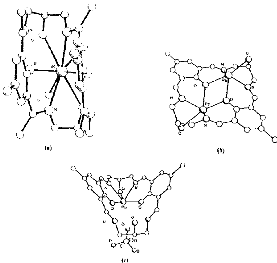
Fig. 107. The structures of (a) \text{Ba}(\text{H}_4\text{-127a})(\text{ClO}_4)_2 (only the coordination oxygen atom of each of the \text{ClO}_4^- ligands is shown), (b) [\text{Pb}_2(\text{H}_2\text{-127a})](\text{ClO}_4)_2 and (c) [\text{Pb}(\text{H}_4\text{-127a})](\text{ClO}_4)_2 .
