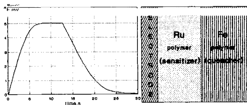
Fig.7 Dependence of \text{Pt, poly-[Ru(5-Clphen)}_3\text{]} | \text{poly-[Fe(5-Clphen)}_3\text{]} system potential upon light irradiation.
