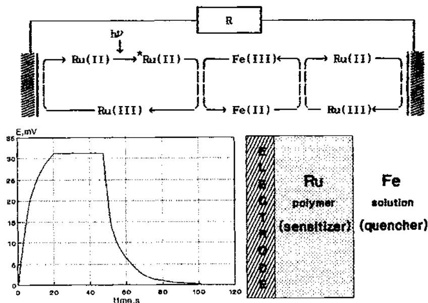
Fig.6 Dependence of \text{Pt, poly-[Ru(5-Clphen)}_3\text{]} | [\text{Fe(phen)}_3]^{3+} system potential upon light irradiation.
