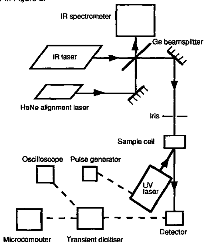
Figure 2. A schematic representation of the TRIR apparatus at Nottingham. The UV pulsed laser generates transients (excited states and/or intermediates). The continuous IR laser monitors the change in transmission at a particular IR wavelength (determined by the IR spectrometer), producing a trace showing change of IR intensity with time. The experiment is repeated at different IR wavelengths and hence a complete IR spectrum of the transient can be built up.
