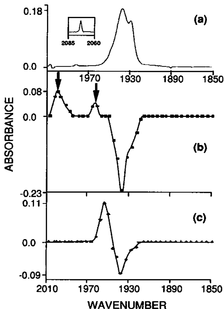
Figure 4 (a) FTIR spectrum of W(CO)_5(4-CNpyr) in methyl cyclohexane (ca. 4 \times 10^{-5} M, pathlength 4 mm); the insert shows the high wavenumber band. TRIR spectra at (b) 150 ns and (c) 5 \mu s , after the dye laser flash (510 nm, 10 ns) of solutions of W(CO)_5(4-CNpyr) in methyl cyclohexane (ca. 4 \times 10^{-5} M, pathlength 5 mm). (Reproduced, with permission, from reference [22]).
