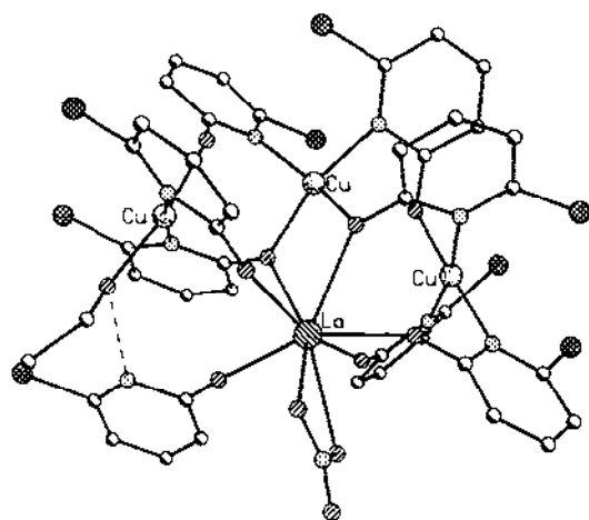
Fig. 39. The structure of [\text{Cu}_3\text{La}(\text{chp})_8(\text{NO}_3)(\text{EtOH})] in the crystal (based on data from ref. 167).
