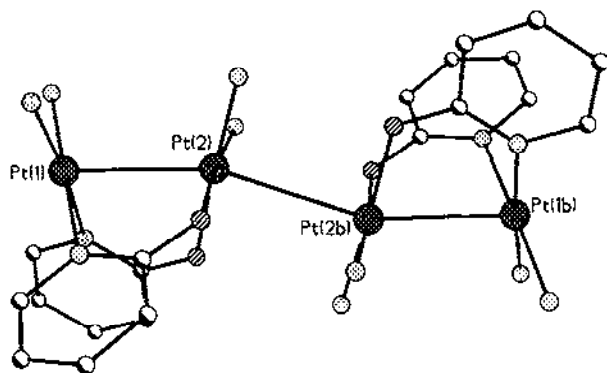
Fig. 26. The structure of the tetranuclear "platinum blue" cation [\text{Pt}_2(\text{NH}_3)_4(\text{hp})_2]^{2+} in the crystal (based on data from ref. 130).
