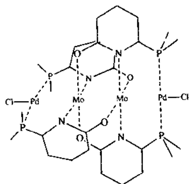
Fig. 8. A schematic diagram showing the structure of the tetranuclear complex [Mo_2Pd_2(php)_4Cl_2] (based on data from ref. 72).
