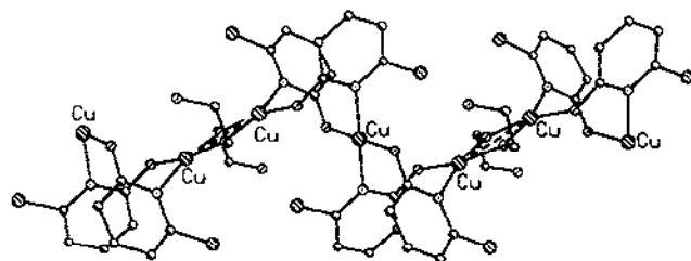
Fig. 31. The structure of the polymeric complex [\text{Cu}_3(\text{chp})_4(\text{OCH}_2\text{CH}_2\text{OH})_2]_n in the crystal (based on data from ref. 55).
