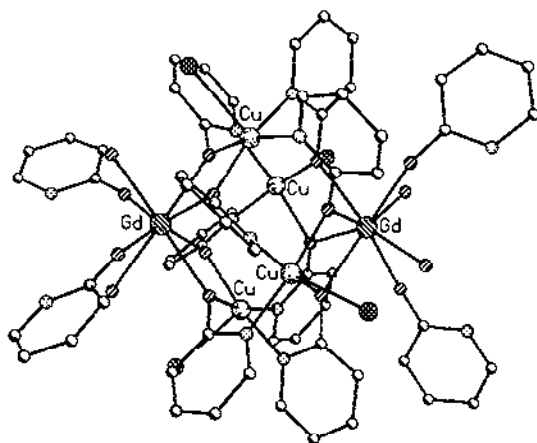
Fig. 37. The structure of the cation [\text{Cu}_4\text{Gd}_2(\text{hp})_6(\text{Hbp})_4\text{Cl}_4(\text{H}_2\text{O})_4]^{2+} in the crystal (based on data from ref. 7).
