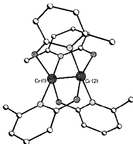
Fig. 4. The structure of [Cr 2 (mhp) 4 ] in the crystal (based on data from ref. 1).
