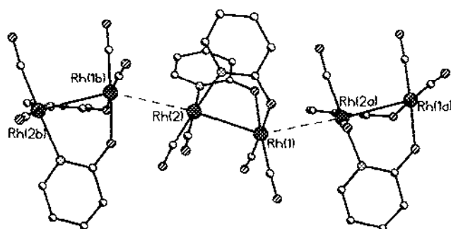
Fig. 21. The stacking of the dimer [\text{Rh}_2(\text{hp})_2(\text{CO})_4] in the crystal (based on data from ref. 123).
