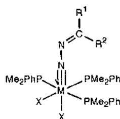
M = Mo, W \text{X} = \text{Cl}, \text{Br}, \text{I}
