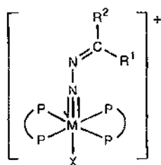
M = Mo, W \text{P} = \text{Ph}_2\text{PCH}_2\text{CH}_2\text{PPh}_2
