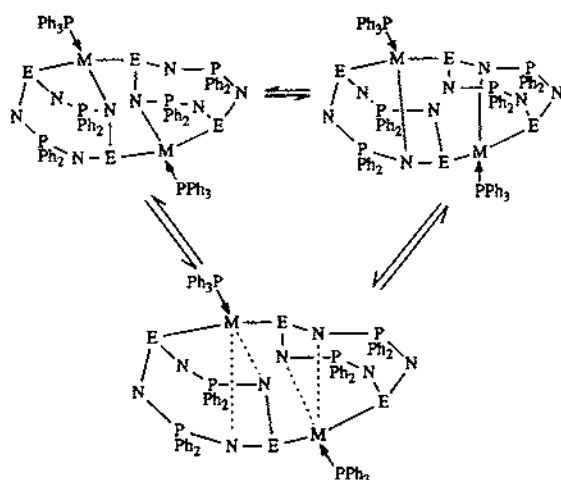
Fig. 1. Proposed mechanism for the [1,3] metallotropic rearrangement in [M(PPh_3)(R_2P_2N_4E_2)]_2 , 22 (M ≡ Pt, Pd; E ≡ S, Se).
