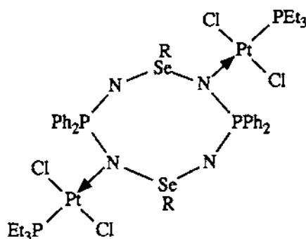
19 ( R \equiv \text{Me, Et, Ph} )
