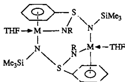
44 (M \equiv Na, K, R + , Cs; R \equiv 'Bu. or SiMe 3 )
