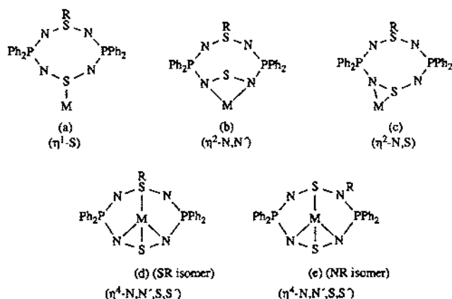
Fig. 6. Coordination modes in metal complexes of \text{Ph}_4\text{P}_2\text{N}_4\text{SR} , where M represents the metal and ancillary ligands. One of the coordinated nitrogens in (b) also serves as a bridge to another metal to give a dimeric structure (see Section 2.3.3 for specific details).
