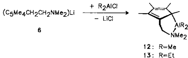
Scheme 9.
