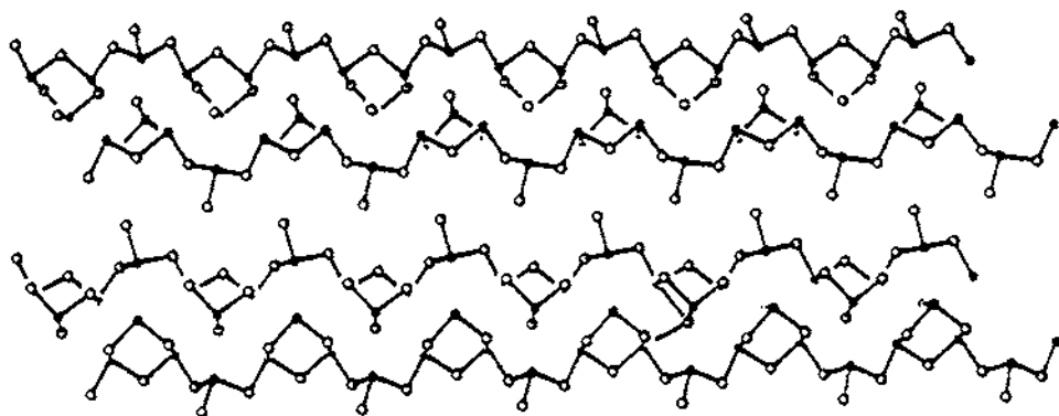
Fig. 29. Computer generated view of the anionic portion of [\text{NH}_4]_2[\text{Sb}_4\text{S}_7] . Note the similarity of the eight-membered rings to those in \text{Cs}_7\text{As}_8\text{S}_{13} . However, they are bridged by \phi\text{-SbS}_3 tetrahedra instead of sulfide, creating an entirely different solid state structure ( \circ , sulfur atoms; \bullet , antimony atoms; ammonium ions not shown) [70].
