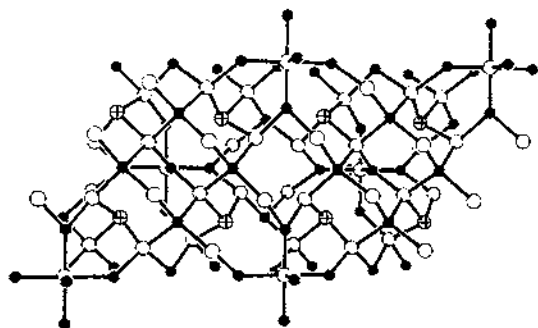
Fig. 16. Computer drawing of several repeat units of \text{Cu}_{12}\text{Sb}_4\text{S}_{13} (tetrahedrite). Note the \phi -pyramidal \text{SbS}_3^- groups linking the Cu(I) groups. Note also the lone \text{S}^{2-} group surrounded by an octahedron of Cu(I) atoms ( \circ , sulfur atoms; \bullet , copper atoms; \oplus , antimony atoms). Coordinates taken from ref. 53.
