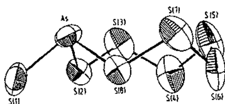
Fig. 27. Thermal ellipsoid plot of [\text{SAsS}_7]^- (reprinted from ref. 67).
