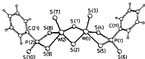
Fig. 41. Thermal ellipsoid view of [W_2S_4(S_2(S)PPh)_2]^{2-} showing the two chelating PhPS_3^- groups (reprinted from ref. 82).
