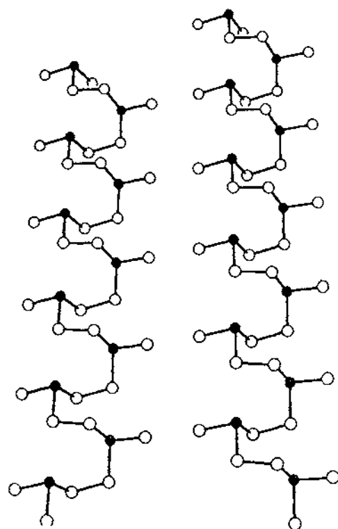
Fig. 21. Computer generated drawing of the anionic portion of \text{KAsSe}_3 showing the double-stranded infinite chains created by the Se-Se bond formation ( \circ , selenium atoms; \bullet , arsenic atoms; potassium ions not shown) [63f].
