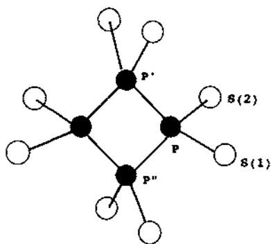
Fig. 9. Thermal ellipsoid plot of \text{P}_4\text{S}_8 [40].
