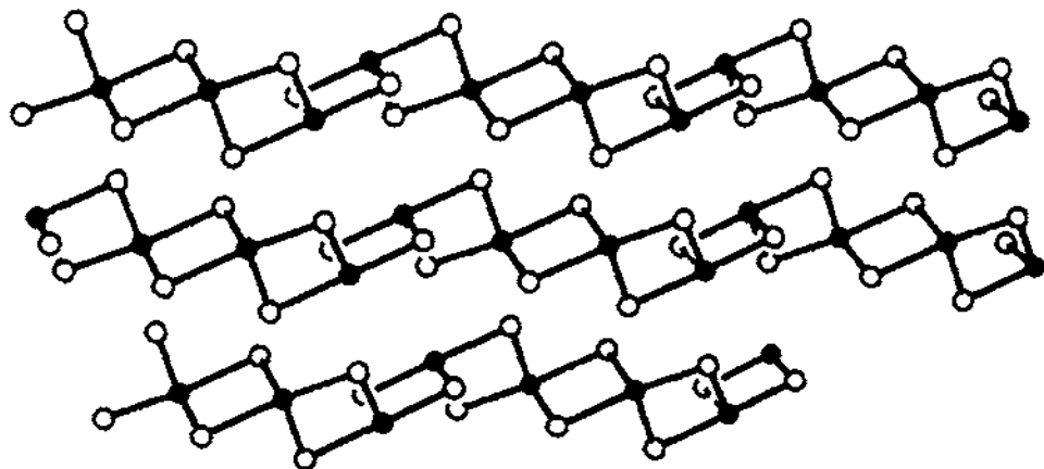
Fig. 12. Computer drawing of KSbSe_2 [47b], showing the infinite chains of antimony selenide between which reside the K^+ ions (○, selenium atoms; ●, antimony atoms, potassium ions not shown).
