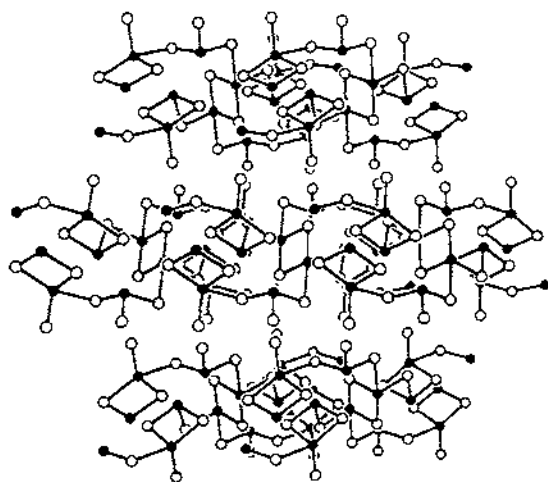
Fig. 14. Computer drawing of the anionic chains of BaSb_2Se_4 showing the edge and corner sharing SbSe_3 and SbSe_4 groups linking together to form an infinite chain [50] ( \circ , selenium atoms; \bullet , antimony atoms; barium atoms not shown).
