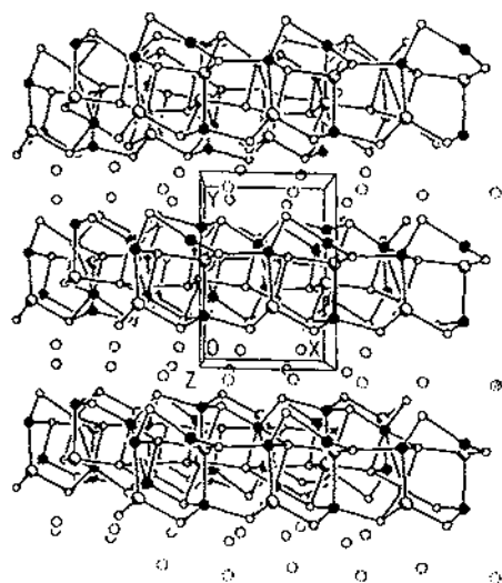
Fig. 25. View of the layered structure of \text{KCu}_2\text{AsS}_3 , showing the \text{AsS}_3^3- groups linking \text{Cu(1)} ions to form layers with \text{K}^+ located between the layers (atoms denoted as in Fig. 24). (reprinted from ref. 66).
