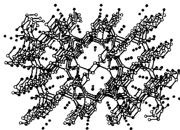
Fig. 24. View of \text{KCu}_4\text{AsS}_4 showing the linking of \text{Cu(I)} ions by \text{AsS}_3^{3-} groups as well as \text{S}^{2-} groups which serve to create a complex channeled structure, with the \text{K}^+ ions located in the channels ( \circ , sulfur atoms; \bullet , copper atoms; \bullet , arsenic atoms; filled circles in channels, potassium ions) (reprinted from ref. 66).
