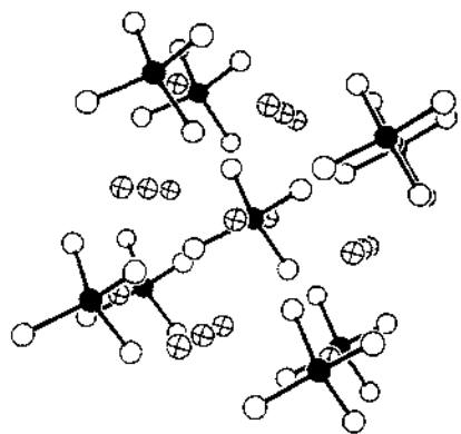
Fig. 13. Computer drawing of K_3SbS_4 [16b] highlighting the large amount of ion pairing between the highly charged anionic clusters and the large number of counterions.
