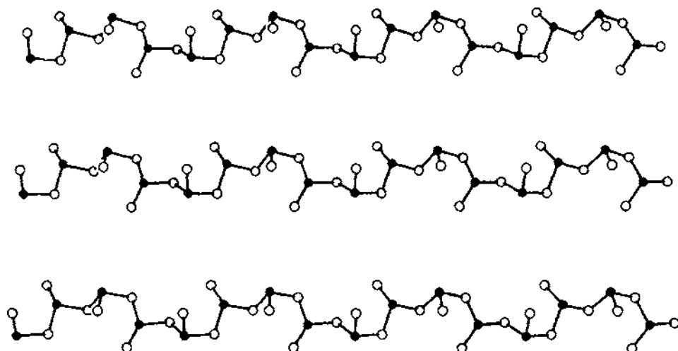
Fig. 26. Computer generated drawing of the anionic portion of \text{KAsSe}_2 . Note the infinite chains created by the corner linking \text{AsSe}_3^{2-} groups (○, selenium atoms; ●, arsenic atoms; potassium ions not shown) [63c].
