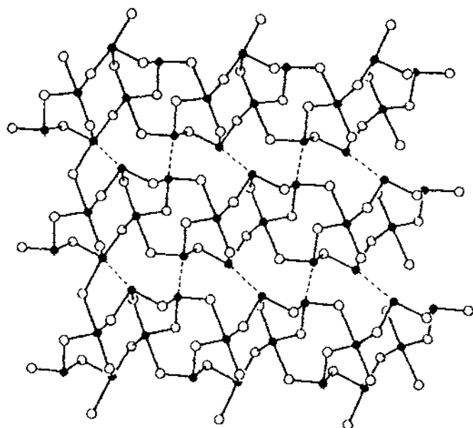
Fig. 31. Computer generated structure of the anionic portion of \text{RbSb}_3\text{Se}_5 , showing the infinite slabs created by the linking of one \phi -tetrahedron and two \phi -trigonal bipyramids ( \circ , selenium atoms; \bullet , antimony atoms; rubidium ions not shown) [63a].
