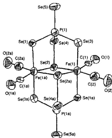
Fig. 38. Thermal ellipsoid view of [\text{Fe}_2(\text{CO})_4(\text{PSe}_3)_2]^{2-} highlighting the two bridging \text{PSe}_3^{3-} units (reprinted from ref. 25).
