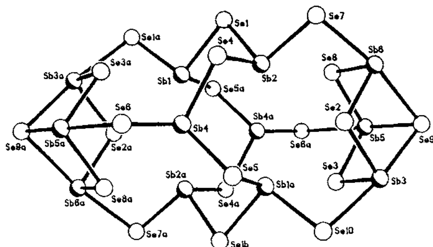
Fig. 8. Thermal ellipsoid plot of \text{Sb}_{12}\text{Se}_{20} [40].
