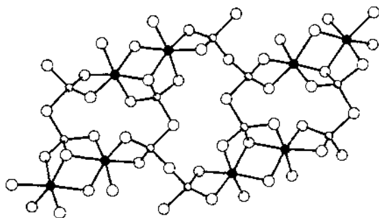
Fig. 17. Computer generated drawing of V_2P_4S_{13} (○, sulfur atoms; ●, vanadium atoms; ◐, phosphorus atoms). Note the bridging P_3S_{10}^{6-} groups linking the metal centers together [55b].
