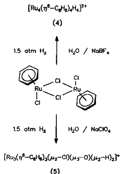
Scheme 2.
