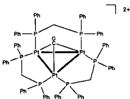
[Pt_3(\mu_3-CO)(\mu_2, \eta^2-Ph_2PCH_2PPh_2)_3]^{2+} (13)
