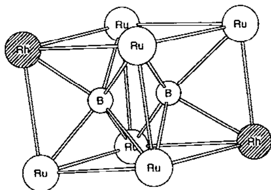
Fig. 26. The \{\text{Rh}_3\text{Ru}_6\text{B}_2\} double prism that constitutes the central core of the [\text{Rh}_3\text{Ru}_6(\text{CO})_{22}\text{B}_2]^- anion.
