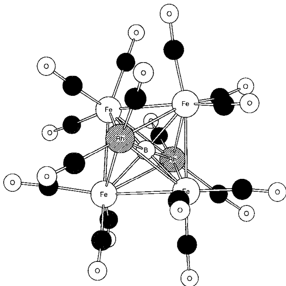
Fig. 25. The structure of the anion trans -[Fe 4 Rh 2 (CO) 16 B] - .
