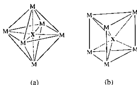
Fig. 1. (a) Octahedral and (b) trigonal prismatic M_6 cages encapsulating an atom X (e.g. X = C or N).
