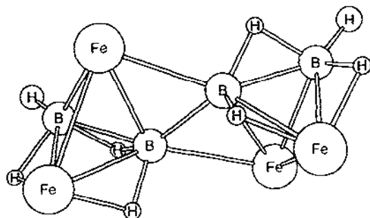
Fig. 27. The coupled cage of one isomer of [\{\text{Fe}_2(\text{CO})_6\text{B}_2\text{H}_4\}_2] (carbonyl ligands omitted) showing fusion utilizing two B–Fe bonds.
