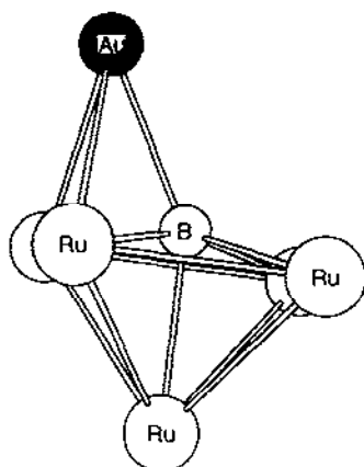
Fig. 19. The \{\text{Ru}_5\text{BAu}\} core of [\text{Ru}_5(\text{CO})_{15}\text{B}\{\text{AuFPh}_3\}] .
