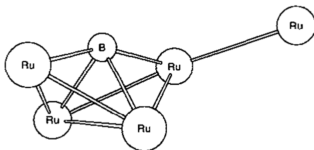
Fig. 6. The \text{Ru}_3\text{B} core of [\text{H}_2\text{Ru}_5(\text{CO})_{13}\text{Cp}^*\text{BH}_2] .
