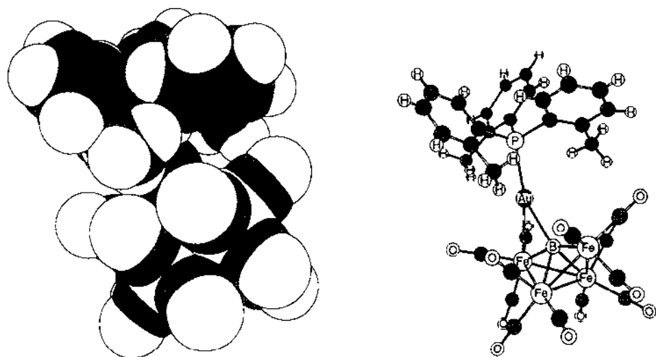
Fig. 14. Two views of the structure of [\text{HFe}_4(\text{CO})_{12}\text{BH}\{\text{AuP}(\text{o-tolyl})_3\}] emphasizing the protective "umbrella" of the bulky phosphine ligand.
