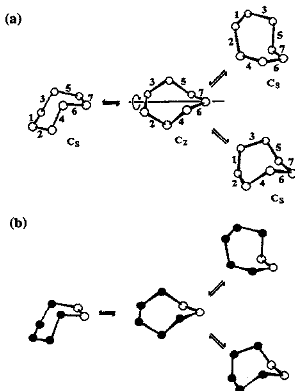
Fig. 15. The pseudorotation scheme in (a) S_7 and (b) 1,2,3,4,5\text{-Se}_5\text{S}_2 [86] (© American Chemical Society).
