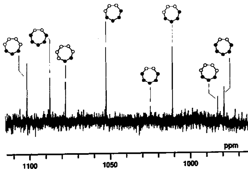
Fig. 18. ^{77}\text{Se} NMR spectrum of \text{Sc}_n\text{S}_{7-n} species prepared by the reaction of [\text{Ti}(\text{C}_5\text{H}_5)_2\text{Se}_n\text{S}_{5-n}] with \text{S}_2\text{Cl}_2 [87] (© Royal Society of Chemistry).
