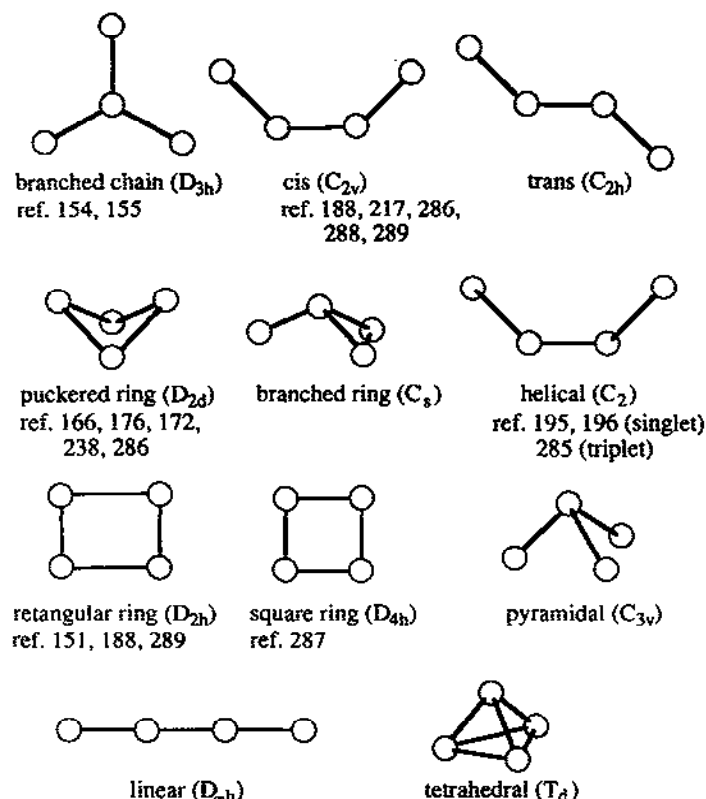
Fig. 21. Isomers of S_4 . The suggestions for the ground-state have also been indicated.
