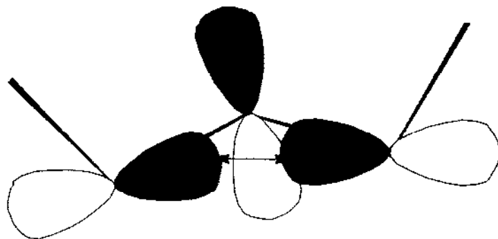
Fig. 10. The orientation of the p lone-pair orbitals in three adjacent chalcogen atoms. Eggert et al. [234] have used these spatial relationships to explain the relative magnitudes of ^1J(\text{SeSe}) and ^2J(\text{SeSe}) coupling constants.
