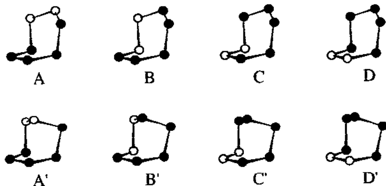
Fig. 16. The different possible isomers of 1,2,3,4,5-Se 5 S 2 in chair and boat conformations [86] (© American Chemical Society).
