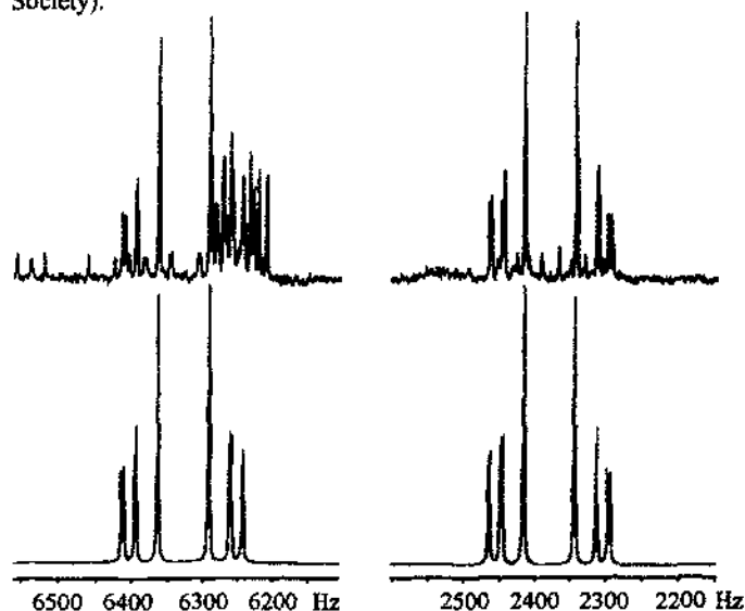
Fig. 8. Observed and calculated spectra of 1,2,3,4-Sc 4 S 4 (A 4 ). The small signals in the middle of the two multiplets are caused by the existence of different isotopomers of significant abundance [226] (© American Chemical Society).
