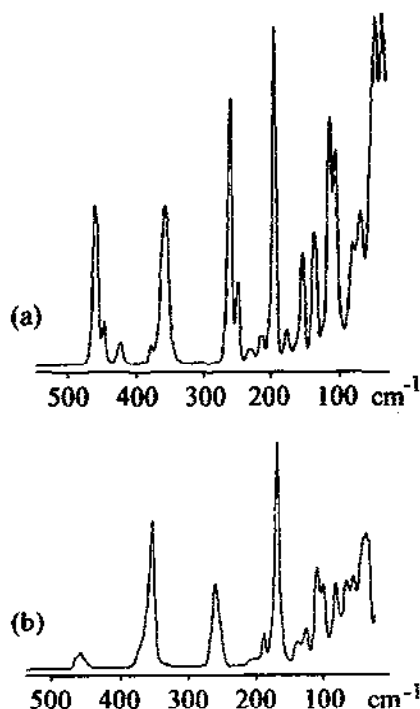
Fig. 5. Low-temperature Raman spectra of (a) 1,2,3- \text{Se}_3\text{S}_5 [85] (© Johann Ambrosius Barth Verlag) and (b) 1,2,5,6- \text{Se}_4\text{S}_4 (adapted from [89], © American Chemical Society).
