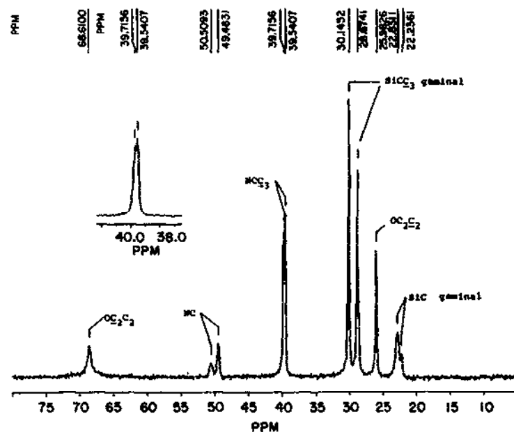
Fig. 5. Solid state ^{13}\text{C} NMR spectra of 11.
