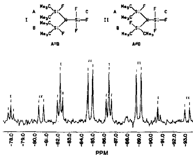
Fig. 18. ^{29}\text{Si} NMR spectrum of 30 ( \text{SiF}_3 group).
