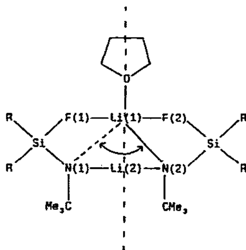
Fig. 6. Structure of 11 in solution.
