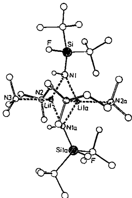
Fig. 2. Crystal structure of [(\text{CMe}_3)_2\text{SiFNHLi}(\text{tmeda})]_2 (5). Si-F 164.3 pm, Si-N 167.2 pm, N-H 82.2 pm.
