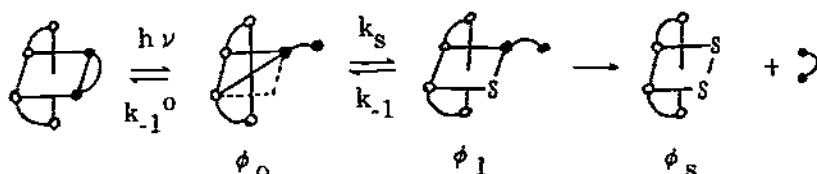
Figure 2. Reaction scheme for the photosubstitution of [\text{Ru}(\text{bpy})_2(\text{dmbpy})]^{2+}
