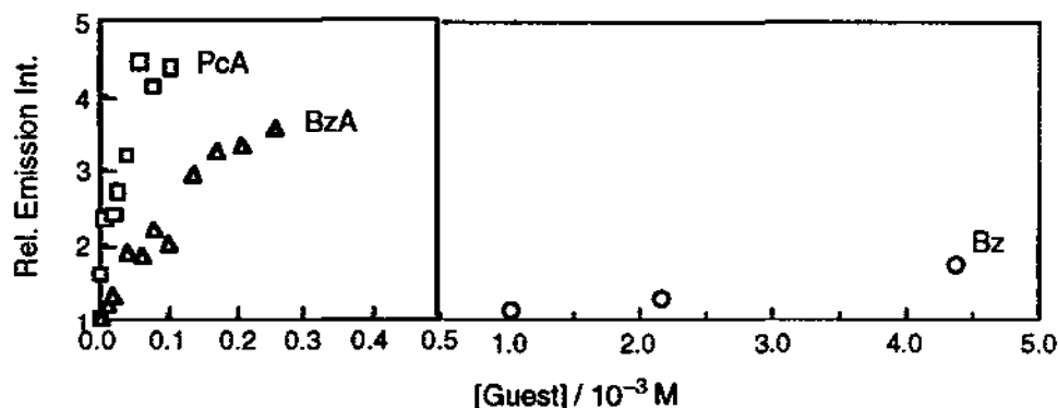
Figure 5. Relative emission intensity from aqueous solutions of \beta -CDU 1 aza \supset Eu 3+ upon addition of light harvesting guests (PcA, picolinic acid; BzA, benzoic acid; Bz, benzene). Please note discontinuity in the abscissa.
