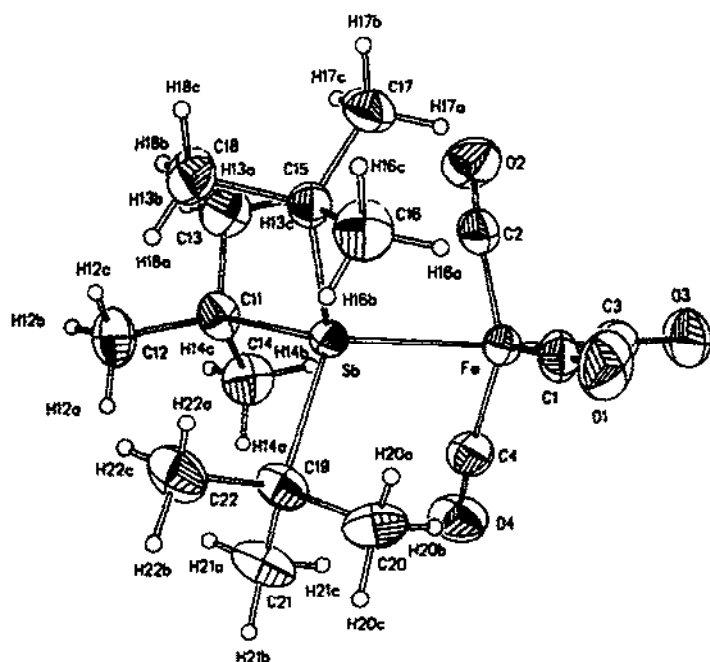
Fig. 2. Molecular structure of \text{Fe(CO)}_4(\text{t-Bu}_3\text{Sb}) . (From ref. 100 by permission of Acta Crystallographica .)
