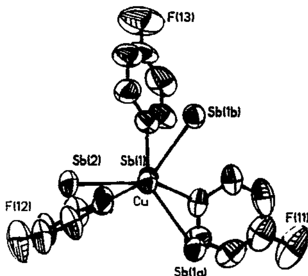
Fig. 23. Molecular structure of [\text{Cu}\{(\text{p-FC}_6\text{H}_4)_3\text{Sb}\}_4]^+ . (From ref. 644 by permission of the American Chemical Society.)
