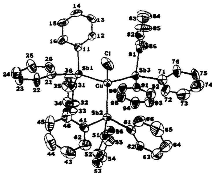
Fig. 22. Molecular structure of \text{CuCl}(\text{Ph}_3\text{Sb})_3 . (From ref. 639 by permission of Plenum Publishing Corporation.)
