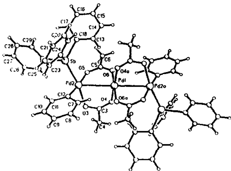
Fig. 21. Molecular structure of \text{Pd}_3(\text{MeCO}_2)_4\text{Ph}_2(\text{Ph}_3\text{Sb})_2 . (From ref. 634 by permission of Pergamon Press Ltd.)
