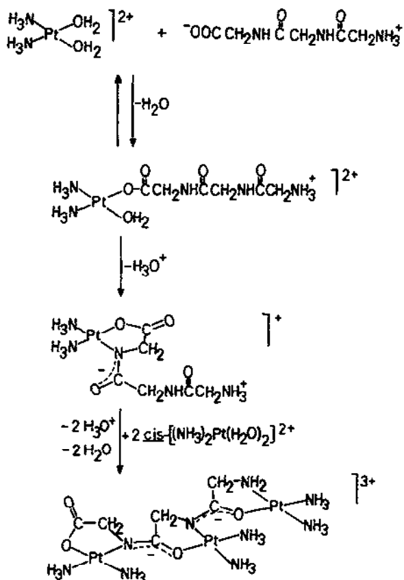
Fig. 18. Interaction of the hydrolysis products of cisplatin with triglycine in aqueous solution.
