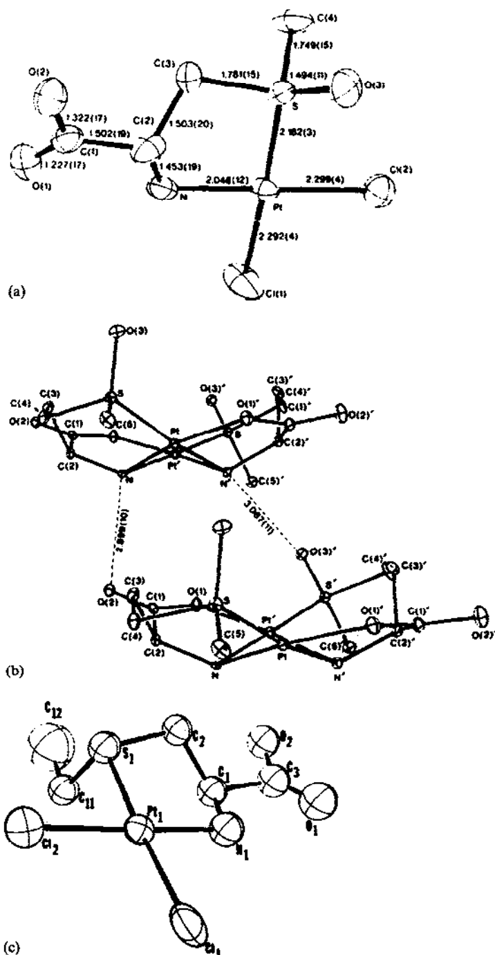
Fig. 21. Molecular structure of Pt(II) complexes with sulphur-containing amino acids. (a) S -oxide of methyleysteine (from ref. 173); (b) S -oxide of S -methionine (from ref. 179); (c) S -ethylcysteine (from ref. 175).
