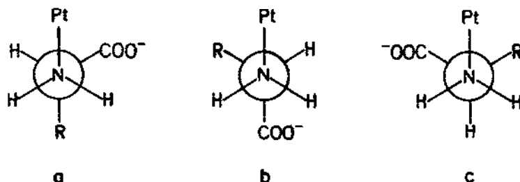
Fig. 5. Rotamers of the coordinated amino acids in \text{trans}[\text{Pt}(\text{amacH})_2(\text{thio})_2]\text{Cl}_2 .
