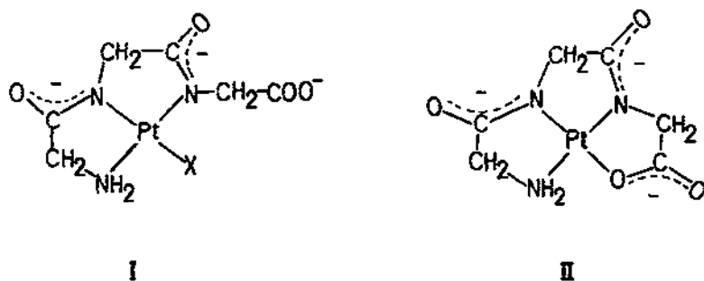
Fig. 17. Products of the interaction of triglycine (gly-gly-gly) with \text{K}_2\text{PtCl}_4 : I, [\text{Pt}\{(\text{gly-gly-gly})\text{-H}_2\}\text{X}]^{2+} ( \text{X} = \text{Cl}^- , \text{OH}^- ); and II, [\text{Pt}\{(\text{gly-gly-gly})\text{-H}_4\}] .
