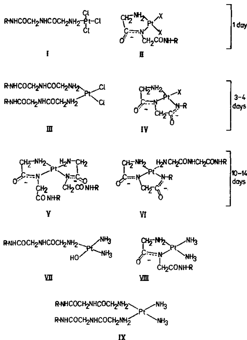
Fig. 7. Products of the reactions of the tripeptide gly-gly-gly with the salts K_2PtCl_4 and cis-(NH_3)_2PtCl_2 ( R = CHCOO^- ; X = Cl^- , OH^- ). The charges on the complexes have been omitted.
