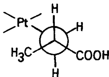
Fig. 2. The amino acid conformation in the complex \text{trans}[\text{Pt}(\text{L-alaH})_2\text{Cl}_2] .
