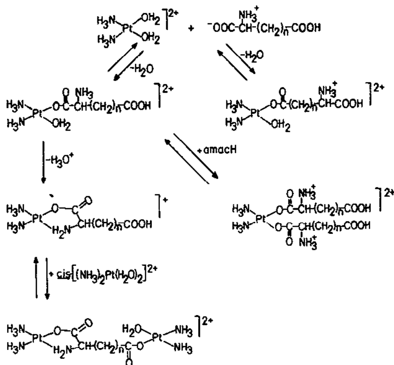
Fig. 15. Interaction of the hydrolysis products of cisplatin with aspartic ( \text{aspH}_2 , n = 1 ) and glutamic acid ( \text{gluH}_2 , n = 2 ) in aqueous solution.
