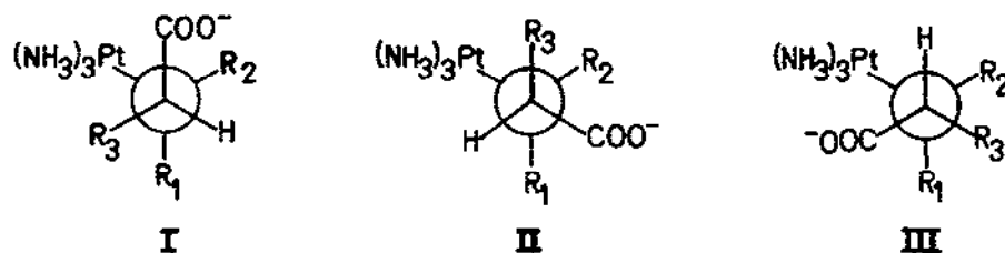
Fig. 3. The three possible rotamers around the \text{N-C}\alpha bond, of an N coordinated to Pt(II) amino acid.
