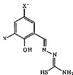
Hsalthsa
