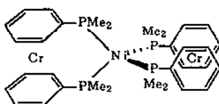
[\text{Cr}(\text{PhPMe}_2)_2]_2\text{Ni}
