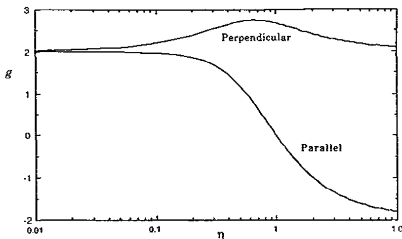
Fig. 7. Predicted g -tensor components for a tetragonally or trigonally distorted octahedral complex as a function of the ratio of the spin-orbit coupling parameter to the distortion splitting, \eta = \lambda/\Delta .
