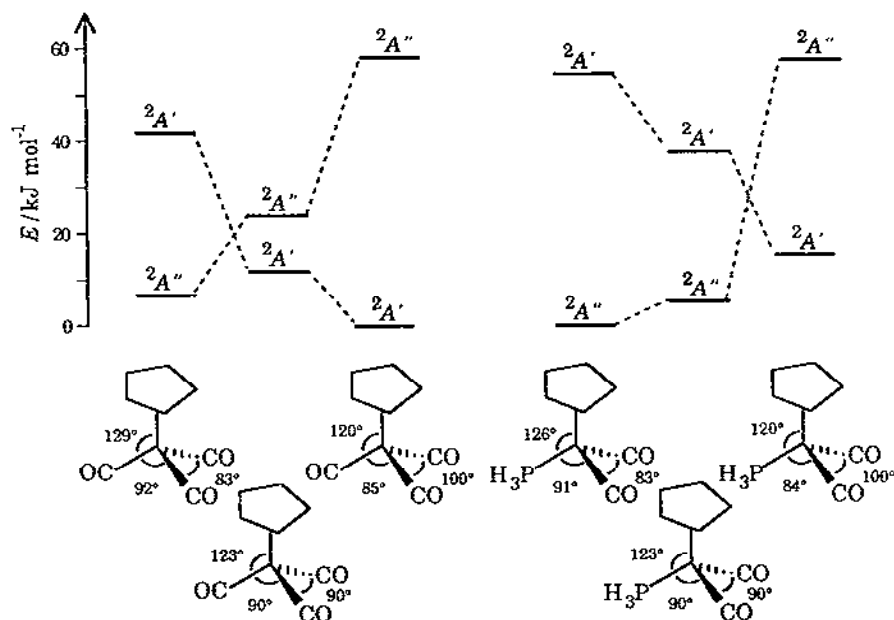
Fig. 2. Relative energies of the ^2A' and ^2A'' states of \text{CpCr(CO)}_3 and \text{CpCr(CO)}_2\text{PH}_3 for the idealized conformation with 90^\circ OC–Cr–CO bond angles and for two minimum-energy conformations retaining C_s symmetry. From Fortier et al. [16].
