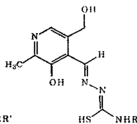
Hpythsa
