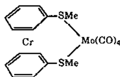
[\text{Cr}(\text{PhSCH}_3)_2]\text{Mo}(\text{CO})_4
