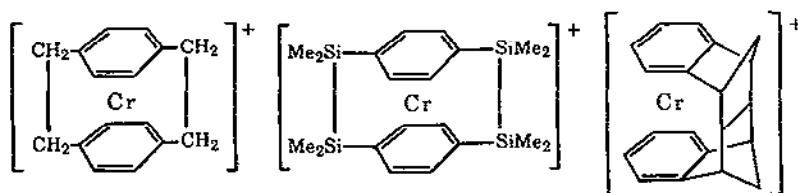
[\text{Cr}([2.2]\text{paracyclophane})]^+ [\text{Cr}(\text{Me}_2\text{SiC}_6\text{H}_4\text{SiMe}_2)_2]^+
