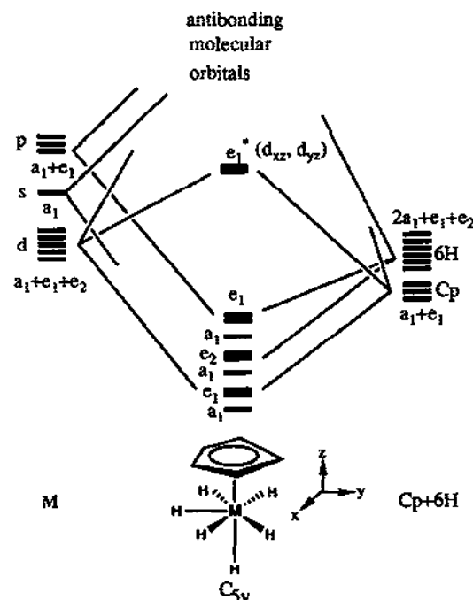
Fig. 4. Molecular orbital interaction scheme for a C 5v CpMH 6 transition metal complex. (Reproduced with permission from Z. Lin and M.B. Hall, Organometallics , 12 (1993) 4046.)
