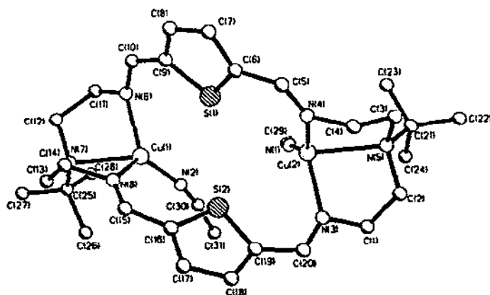
Fig. 12. The synthesis of the dicopper(I) complex (22).
