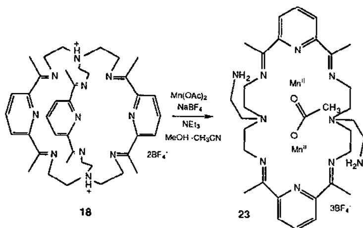
Fig. 14. Synthesis of the dimanganese(II) complex ( 23 ).
