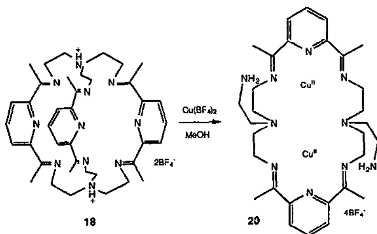
Fig. 11. Synthesis of the dicopper(II) complex (20).
