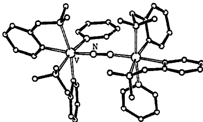
Fig. 2. Structure of the first stable V^{II} dinitrogen complex, 2 , obtained from [VCl_2(tmeda)_2] by substitution of chlorides by the C,N-chelating ligand 1,3- C_6H_4CH_2NMe_2 [44].
