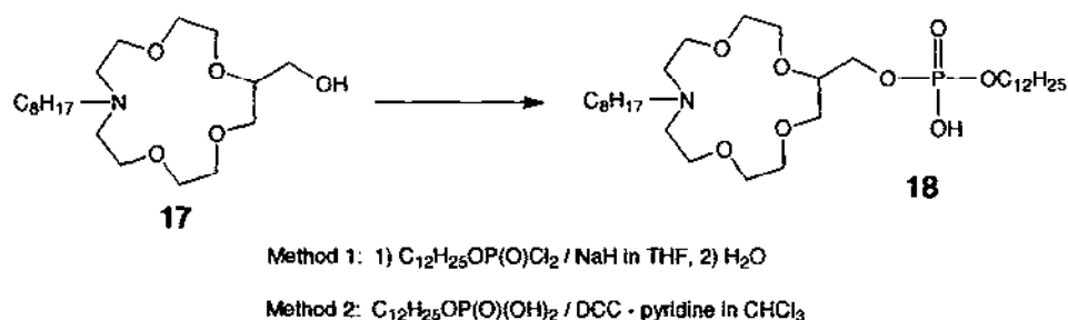
Fig. 6. Monoaza-15-crown-5 with an alkylphosphoric acid functional group. Adapted from Hetero Corporation.
