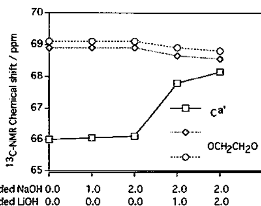
Fig. 14. Titration profile of 8 on addition of NaOH and LiOH. Reproduced with permission from The American Chemical Society.
