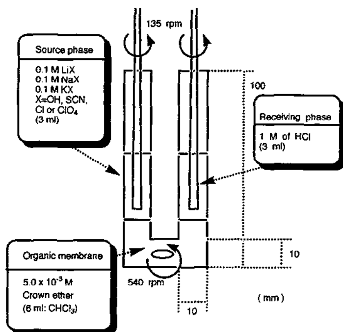
Fig. 7. U-tube cell for transport experiments. Adapted from Elsevier Science Publishers.
