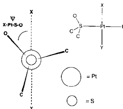
Fig. 7. Scheme of the square planar Pt^{2+} complexes with one S-coordinated sulfoxide. The absolute values of the torsional angles X-Pt-S-O and Y-Pt-S-O are considered to describe the stereochemistry of S-coordination. Among them, for simplicity, only that with the lowest absolute value is taken into account, the other one being nearly supplementary.
