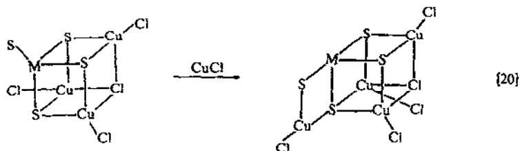
Scheme 4(c). 4 + 1 reactions.
