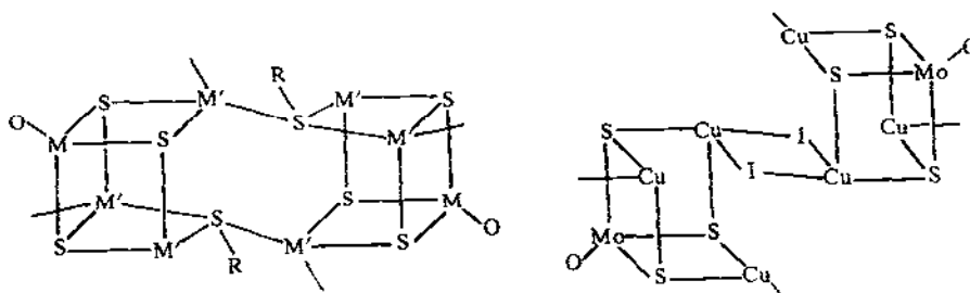
Fig. 12. Octanuclear clusters.
