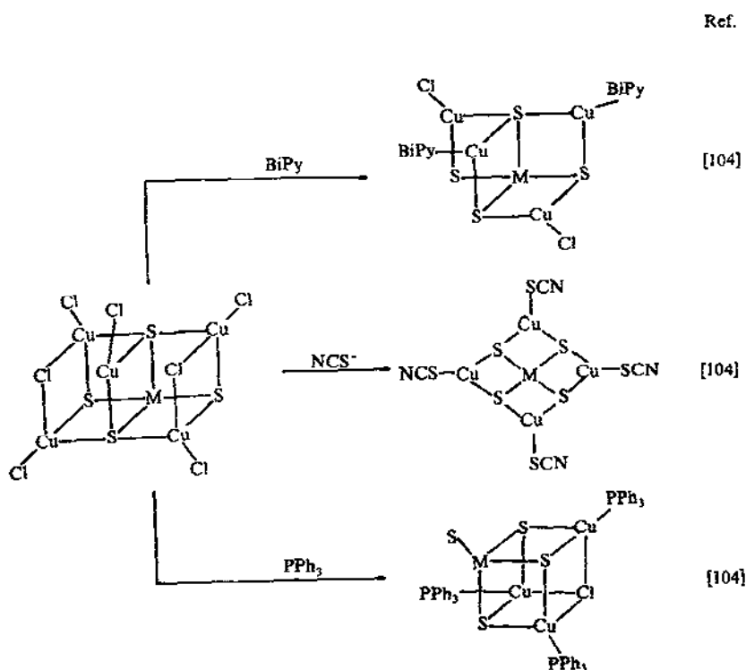
Scheme 5. Decomposition reaction.
