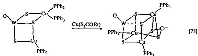
Scheme 4(b). 3 + 1 reactions.
