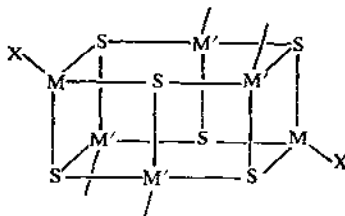
Fig. 10. Hexanuclear clusters.
