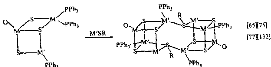
Scheme 4(d). (3+1)+(3+1) reactions.
