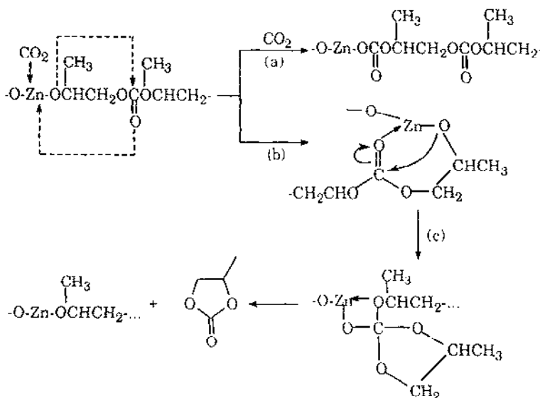
Scheme 8.
