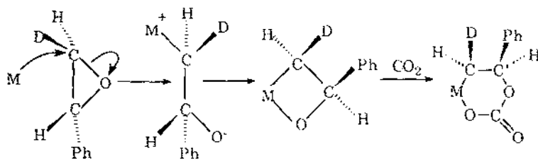
Scheme 12.
