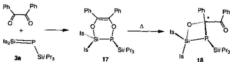
Scheme 6. Synthesis of 17 and 18 .
