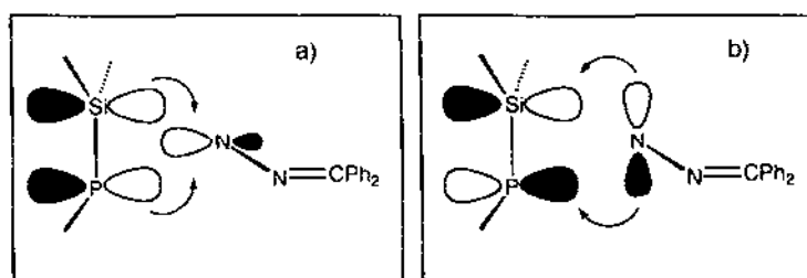
Scheme 8. Description of 24 as \pi -complex (Dewar-Chart-Duncanson model). (a) Si=P bond as \pi -donor, (b) Si=P bond as \pi -acceptor.
