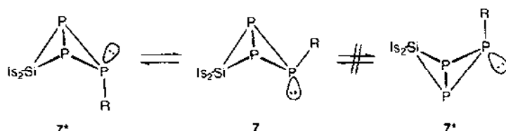
Scheme 4. Isomerization of 7 by phosphorus inversion.
