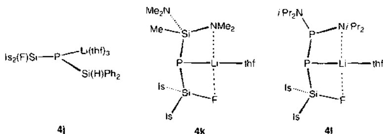
Scheme 3. Lithium-(fluorosilyl)phosphanides 4j–k.
