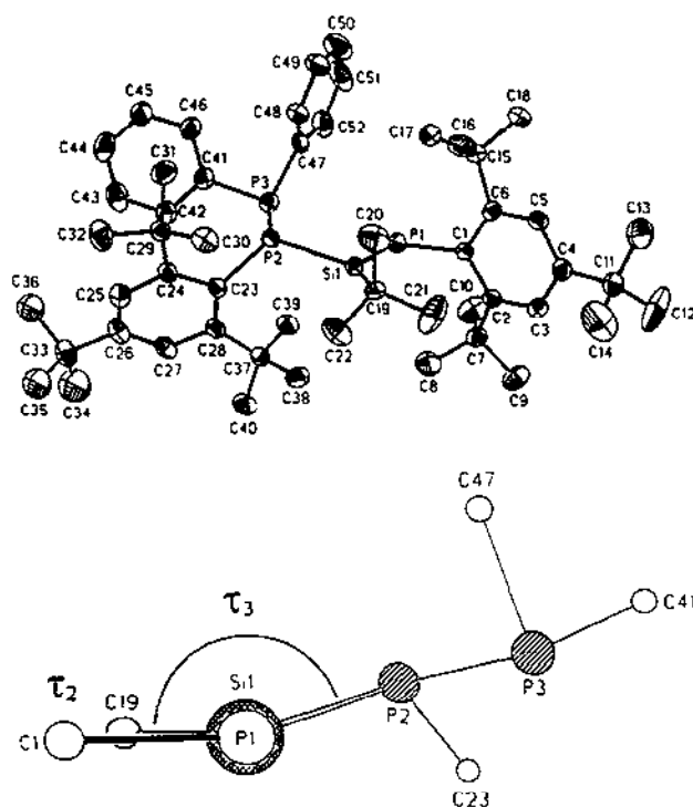
Fig. 5. Solid state structure of 2 , T_2 , \angle \text{C1-P1-Si1-C19} , 3.4(3)^\circ ; T_3 , \angle \text{C1-P1-Si1-P2} , 161.0(2)^\circ .
