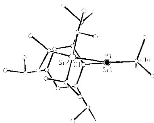
Fig. 7. View of 3i along the Si=P vector.
