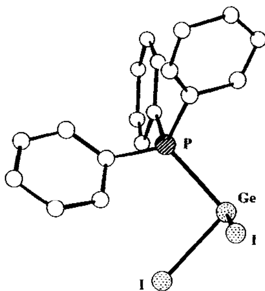
Fig. 5. Molecular structure of [GeI 2 (PPh 3 )] ( 33 ).
