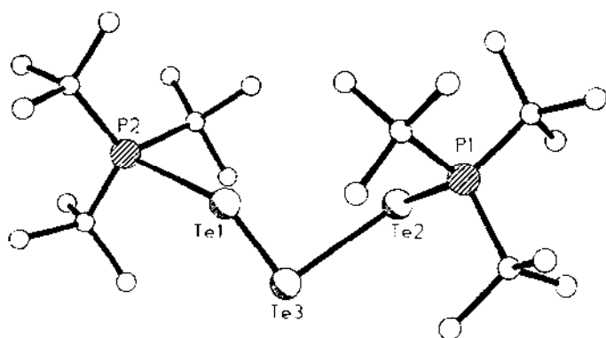
Fig. 12. Molecular structure of the cation [\text{Bu}_3\text{PTe}_3\text{PBu}_3]^{2+} in 53 .
