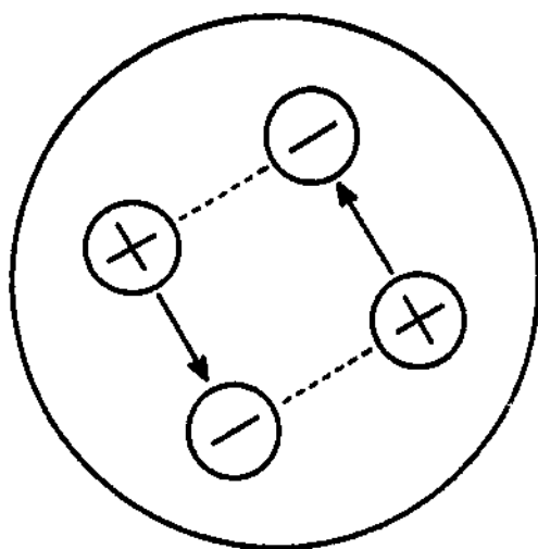
Fig. 1.11. Schematic drawing of a quadrupole moment.
