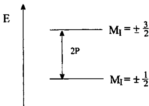
Fig. 1.12. The energy levels of a spin l = \frac{3}{2} at zero magnetic field in axial symmetry, with P being the product of the quadrupole moment with the electric field gradient.
