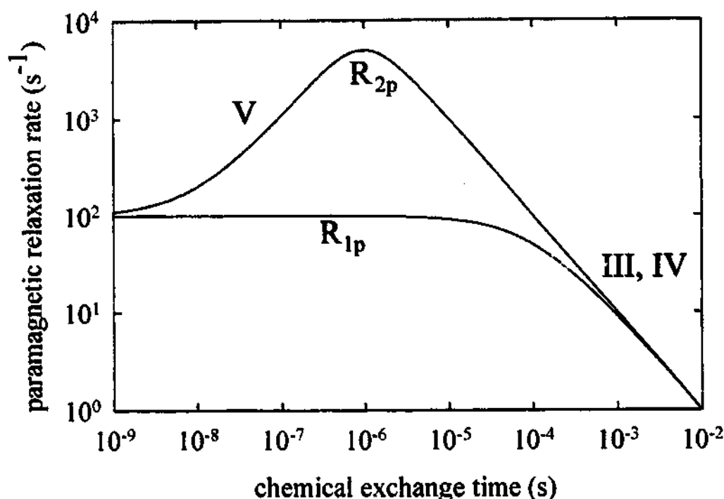
Fig. 4.4. Linear dependence of R_{1p} and R_{2p} (log scale) on \tau_M (log scale) in the exchange regions corresponding to Cases III to V. Conditions: R_{M1} = 10^4 \text{ s}^{-1} , f_M = 10^{-2} , and \Delta\omega_M = 10^6 \text{ rad s}^{-1} .
