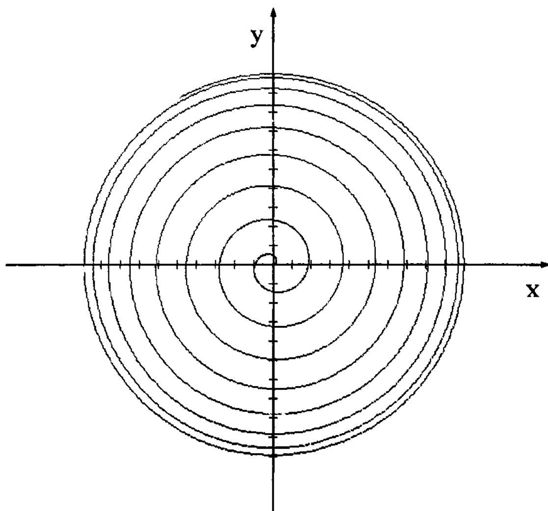
Fig. 9.2. Saturation effect of the modified DANTE sequence on a slightly off-resonance with respect to the carrier frequency. The trajectory of the in-plane component of the magnetization is shown. The z magnetization is tilted by the first small angle pulse toward the x axis, and starts precessing toward the y axis. The duration of the pulse corresponds to the duration of a 90^\circ precession, so that at the end of the first pulse the projection lies on the y axis. The phase of the following pulses is rotated in phase with the precession of the signal, in such a way as to "follow" the spin magnetization in its spiral movement toward the xy plane.
