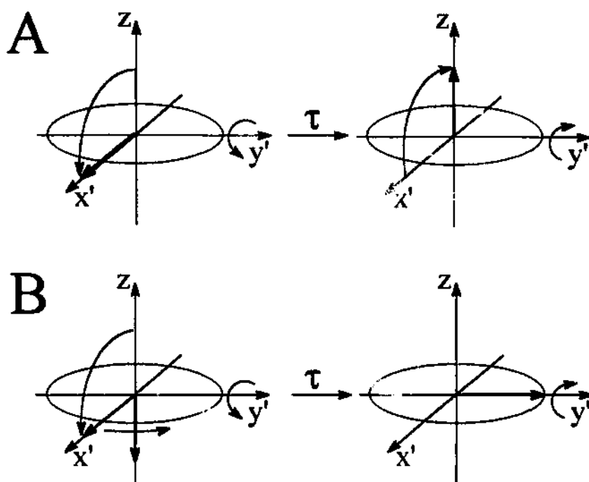
Fig. 9.3. Effect of the JI sequence on a signal on resonance (A) and off-resonance by 1/2\tau Hz (B).
