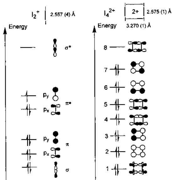
Fig. 54. The 5 \pi MOs of I_2^+ and [I_4]^{2+} .
