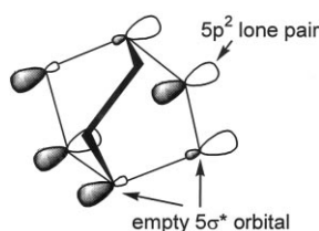
Fig. 45. MO representation of two of the six equivalent 5p^2 \rightarrow 5\sigma^* interactions in the bicyclo[2.2.2]octane structure of \text{Te}_8^{2+} in [\text{Te}_6^{2+}][\text{Te}_8^{2+}][\text{WCl}_6]_4 [13b].
