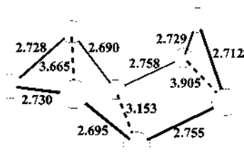
Fig. 8. Solid state structure of the isolated, discrete \text{Te}_8^{2+} dication as found in [\text{Te}_8^{2+}][\text{ReCl}_6^{2-}] [104]. Distances are given in (Å).
