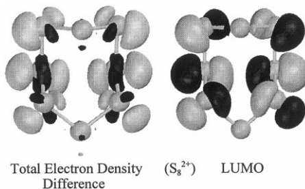
Fig. 38. The LUMO of S_8^{2+} and the total electron density difference of S_8 and S_8^{2+} (both in the C_s symmetric S_8^{2+} minimum geometry). Lighter shaded areas represent electron density left over from S_8 while the darker shaded areas represent electron density left over from S_8^{2+} . (Reprinted with permission from [16], Copyright 2000 American Chemical Society.)
