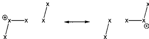
Fig. 56. Valence bond representation of the bonding in X_5^+ .
