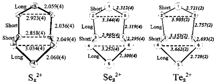
Fig. 35. Experimental bond lengths (averaged assuming local C_s symmetry) and bond alternation in the isostructural E_8^{2+} dication in \text{S}_8(\text{AsF}_6)_2 , (\text{Se}_8)(\text{Te}_6)(\text{AsF}_6)_6 and \text{Te}_8(\text{ReCl}_6) . Distances are given in Å. (Reprinted with permission from [16], Copyright 2000 American Chemical Society.)
