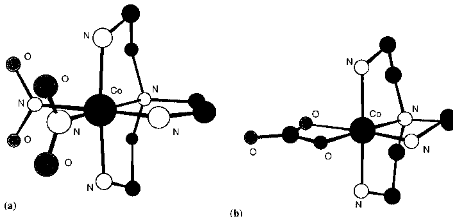
Fig. 1. The MM2 minimised structure of (a) [Co(tren)(NO 2 ) 2 ] + and (b) [Co(tren)CO 3 ] + .
