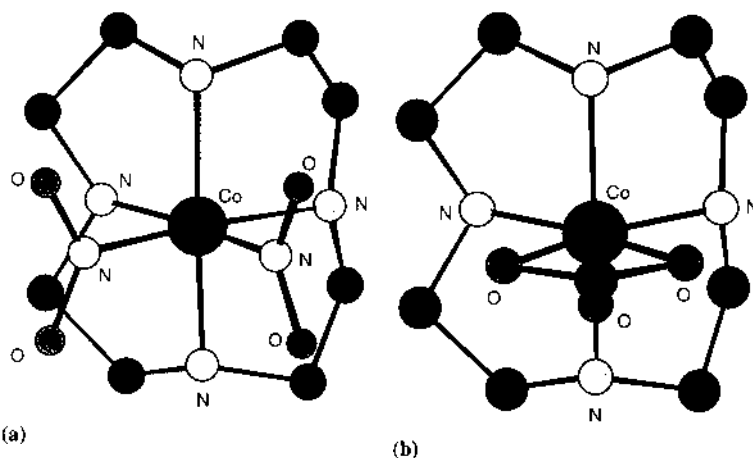
Fig. 2. The MM2 minimised structure of (a) [Co(cyclen)(NO 2 ) 2 ] + and (b) [Co(cyclen)CO 3 ] + .
