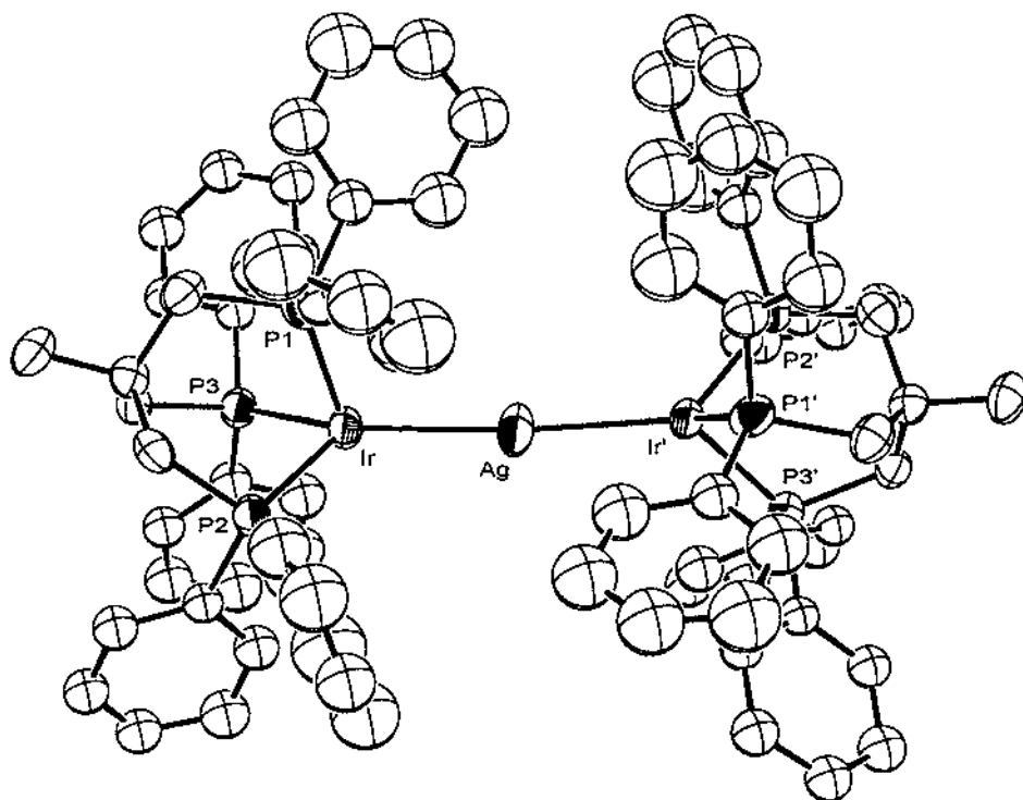
Fig. 5. An ORTEP view of the cation in [(triphos)HIr(μ-H) 2 Ag(μ 2 -H)IrH(triphos)](CF 3 SO 3 ) ( 14 IrAgIr ).
