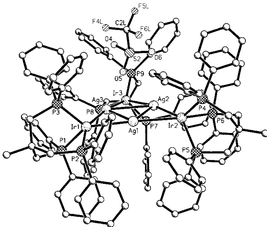
Fig. 12. A view of the interaction between the silver cations and the \text{CF}_3\text{SO}_3^- anion in [(\text{triphos})\text{HIr}(\mu\text{-H})_2\text{Ag}]_3\text{CF}_3\text{SO}_3](\text{CF}_3\text{SO}_3)_2 ( 28 , \text{Ir}_3\text{Ag}_3 ).
