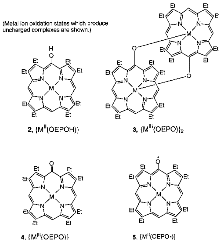
Scheme 3. Basic types of coordination. (Metal ion oxidation states which produce uncharged complexes are shown.)
