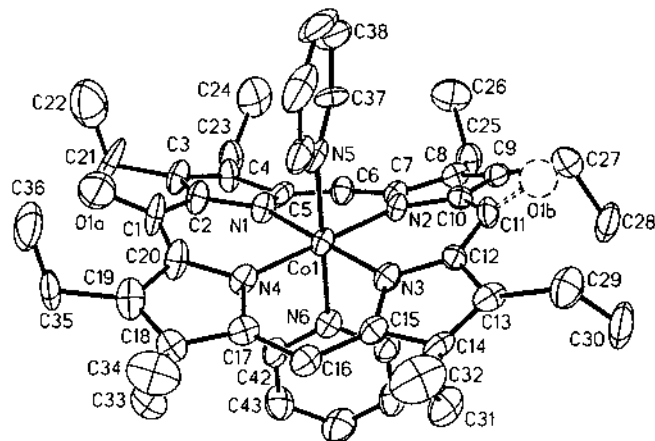
Fig. 5. A view of the crystallographically determined structure of \{(\text{py})_2\text{Co}^{\text{III}}(\text{OEPO})\} with 50% thermal contours. Note the non-planarity of the macrocycle which contrasts with that of shown in Fig. 4. Taken from Balch et al. [17].
