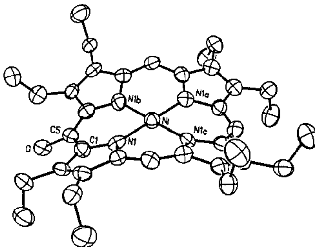
Fig. 2. A drawing of the crystallographically determined structure of \{Ni^{II}(OEPOH)\} (with 50% thermal contours), which has crystallographically imposed S_4 symmetry. There is disorder in the location of the meso -hydroxyl group and only one of the four, equally occupied sites is shown. Taken from Balch et al. [18].
