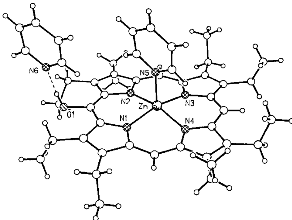
Fig. 1. The crystallographically determined structure of \{(py)Zn^{II}(OEPOH \cdots py)\} . The in-plane Zn–N distances are: N1, 2.093(9); N2, 2.064(8); N3, 2.060(9); and N4, 2.099(8) while the Zn–N5 distance is 2.183(8) Å. Taken from Balch et al. [16].
