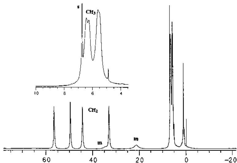
Fig. 12. The 300 MHz ^1\text{H} NMR spectrum of \{\text{Br}_2\text{Fe}^{\text{III}}(\text{OEPOx})\} in chloroform- d solution at 24^\circ\text{C} . Insert A shows an expanded section of the methyl resonances in the 10–4 ppm region. Taken from Balch et al. [27].
