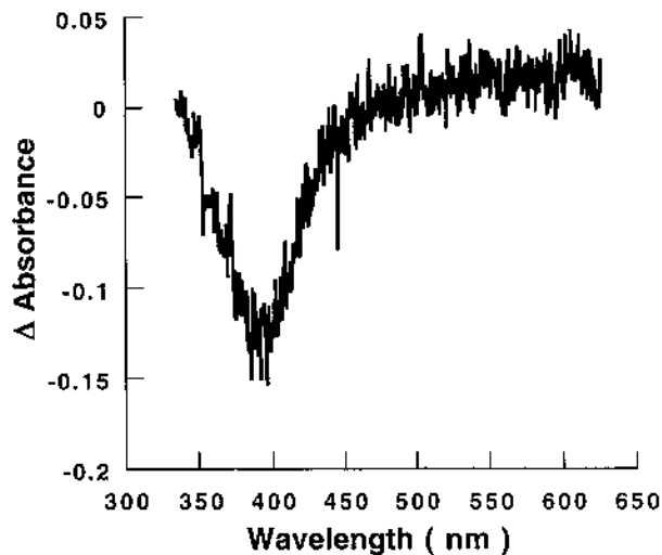
Fig. 3. UV-vis transient absorption by CCD camera. Red Roussin's salt ( 60 \mu\text{M} ) aqueous solution. Gate width = 10 \mu\text{s} , Gate delay = 20 \text{ ns} ; \lambda_{\text{pump}} = 355 \text{ nm} . \Delta\text{Abs} is referenced to the initial absorbance prior to the flash.
