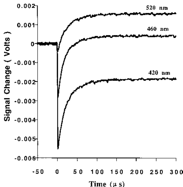
Fig. 2. Transient signal changes upon flash photolysis of \text{Na}_2[\text{Fe}_2\text{S}_2(\text{NO})_4] solution ( 40 \mu\text{M} ) in aerated water, 296 \text{ K} . Various \lambda_{\text{mon}} ( \lambda_{\text{irr}} = 355 \text{ nm} ). Signal changes rather than absorption changes are used to emphasize qualitative differences.
