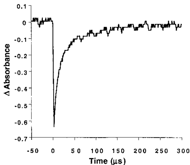
Fig. 4. Transient absorption upon flash photolysis of \text{Na}_2[\text{Fe}_2\text{S}_2(\text{NO})_4] solution ( 40 \mu\text{M} ) in water under argon, 296 \text{ K} ( \lambda_{\text{mon}} = 420 \text{ nm} ; \lambda_{\text{irr}} = 355 \text{ nm} ).
