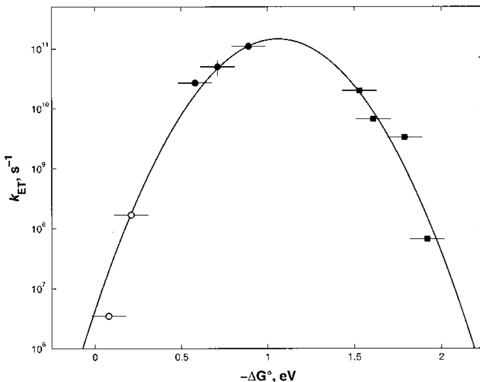
Fig. 3. Driving-force dependence of the [\text{IrPOpy}^+]_2 excited-state ( ^1k_{\text{ET}}^* , ●; ^3k_{\text{ET}}^* , ○) and ground-state ( ^bk_{\text{ET}} , ■) ET rates; the solid line is a fit to Eq. (1) with \lambda = 1.06 eV and H_{\text{AB}} = 24 \text{cm}^{-1} .
