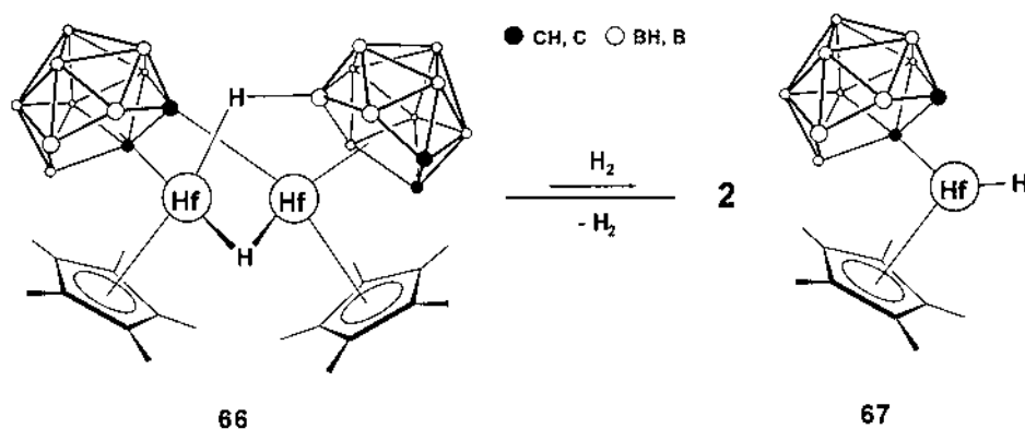
Fig. 17. Formation of a catalytically active mononuclear Hf hydride from the dimer 66 via hydrogenation (ref. [58]).
