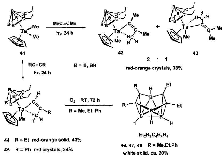
Fig. 14. Insertion of alkynes into the \text{CpMeTa}(\text{carborane}) complex 41 and formation of tetracarborane carboranes via oxidation of vinyl-Ta products 42–45 (ref. [49]).
