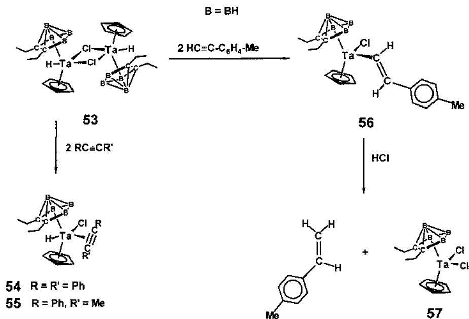
Fig. 16. Reactions of [CpTa(H)Cl(Et_2C_2B_4H_4)]_2 ( 53 ) with alkynes (ref. [53]).
