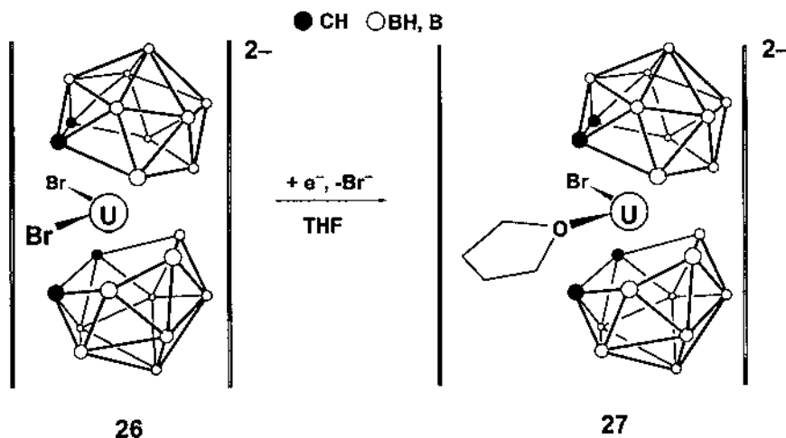
Fig. 10. Reductive interconversion of bis(dicarbollyl) uranium complexes (ref. [38b]).
