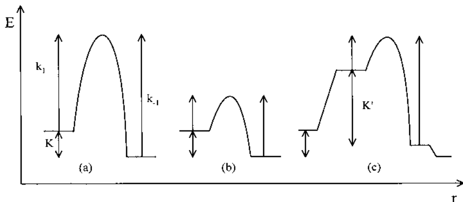
Fig. 1. Kinetics ( k_1 , k_{-1} ) and thermodynamics ( K ) of a single-step chemical reaction; (a) uncatalyzed; (b) catalyzed (conventional model); (c) catalyzed by entasis, the substrate complexation and decomplexation is also included in this case ( K vs. K' , see text).
