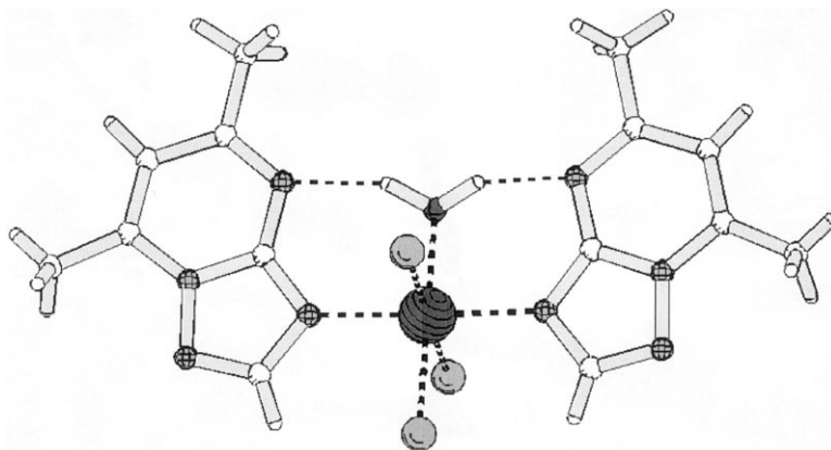
Fig. 31. Drawing of the structure of [\text{Ru}(\text{dntp})_2(\text{H}_2\text{O})\text{Cl}_3] showing the double hydrogen bond from coordinated the water ligand [196].
