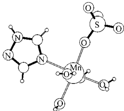
Fig. 5. Monodentate coordination of 1,2,4-triazole in [\text{Mn}(\text{Htrz})(\text{H}_2\text{O})_4\text{SO}_4] [95].
