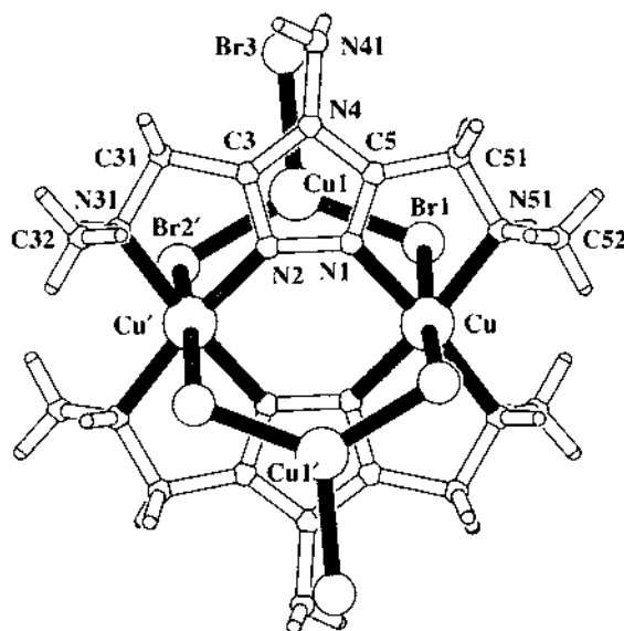
Fig. 24. Projection of the structure of [\text{Cu}_2(\text{maamt})_2(\text{CuBr}_3)_2] showing the stacking of \text{CuBr}_3 anions with triazole rings [32,165].
