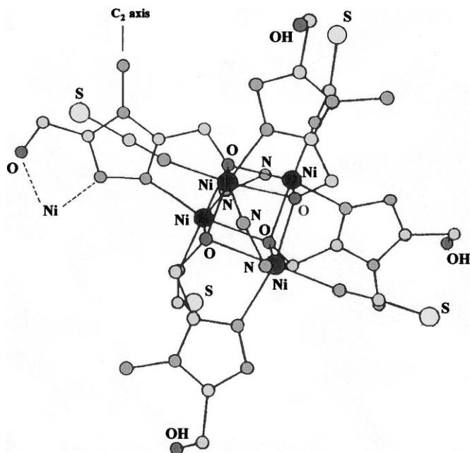
Fig. 25. Schematic drawing of one cubane cluster of the octanuclear double-cubane compound of composition [\{\text{Ni}_4(\text{H}_2\text{ahmt})_2(\text{Hahmt})_3(\text{NCS})_4\}_2(\text{ahmt})]\cdot 12\text{H}_2\text{O} [172]. The doubly deprotonated ligand ahmt is on the two-fold axis bridging two cubane clusters. Of the two neutral ligands \text{H}_2\text{ahmt} only the \text{N}1, \text{N}2 bridges are shown.
