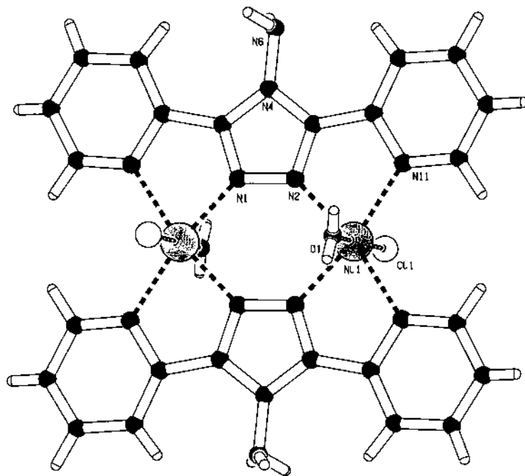
Fig. 21. Skeletal drawing of the structure of the cation of [\text{Ni}_2(35\text{Py}_2\text{atrz})_2(\text{H}_2\text{O})_2\text{Cl}_2]\text{Cl}_2 \cdot 4\text{H}_2\text{O} [155].
