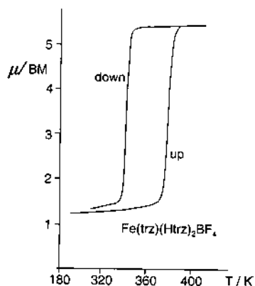
Fig. 4. Magnetic moment vs. temperature of [\text{Fe}(\text{trz})(\text{Htrz})_2]\text{BF}_4 [22].
