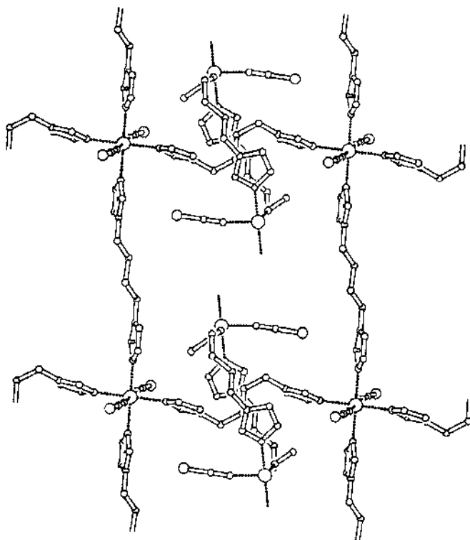
Fig. 20. Representation of the structure of [\text{Fe}(\text{btb})_2(\text{NCS})_2]_\infty , btb = 1,4-bis(triazol-1-yl)butane. Connecting ligands in one direction of a 2d-grid are embraced by the double bridges of 1d-chains [123].
