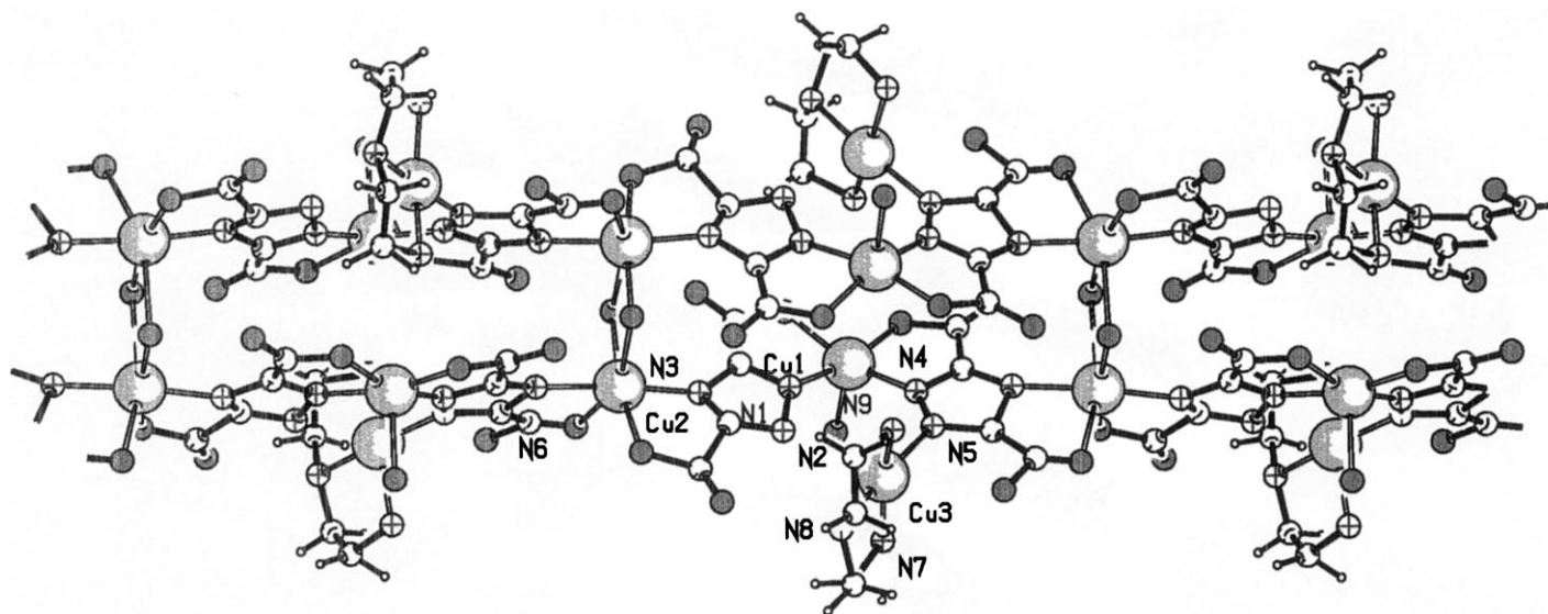
Fig. 27. Representation of the chain structure of [\text{Cu}_3(\text{tdca})_2(\text{dien})(\text{H}_2\text{O})_2 \cdot 3\text{H}_2\text{O}]_\infty , \text{H}_3\text{tdca} = triazole-3,5-dicarboxylic acid [173].
