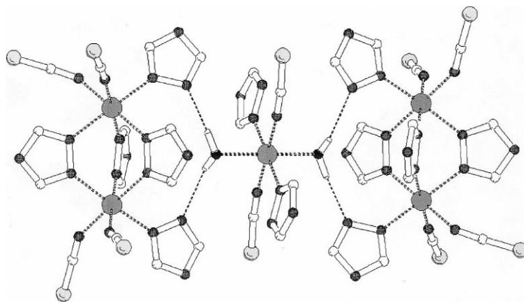
Fig. 12. The pentanuclear assembly [\text{Fe}_2\text{L}_5(\text{NCS})_4]_2[\text{FeL}_2(\text{NCS})_2(\text{H}_2\text{O})_2] , \text{L} = 4\text{-}p\text{-tolyltriazole} ; tolyl groups and CH bonds omitted for clarity [123].
