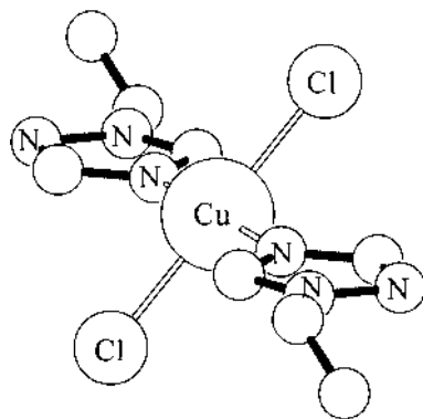
Fig. 19. Molecular structure of [\text{Cu}(\text{1Ettrz})_2\text{Cl}_2] [140].
