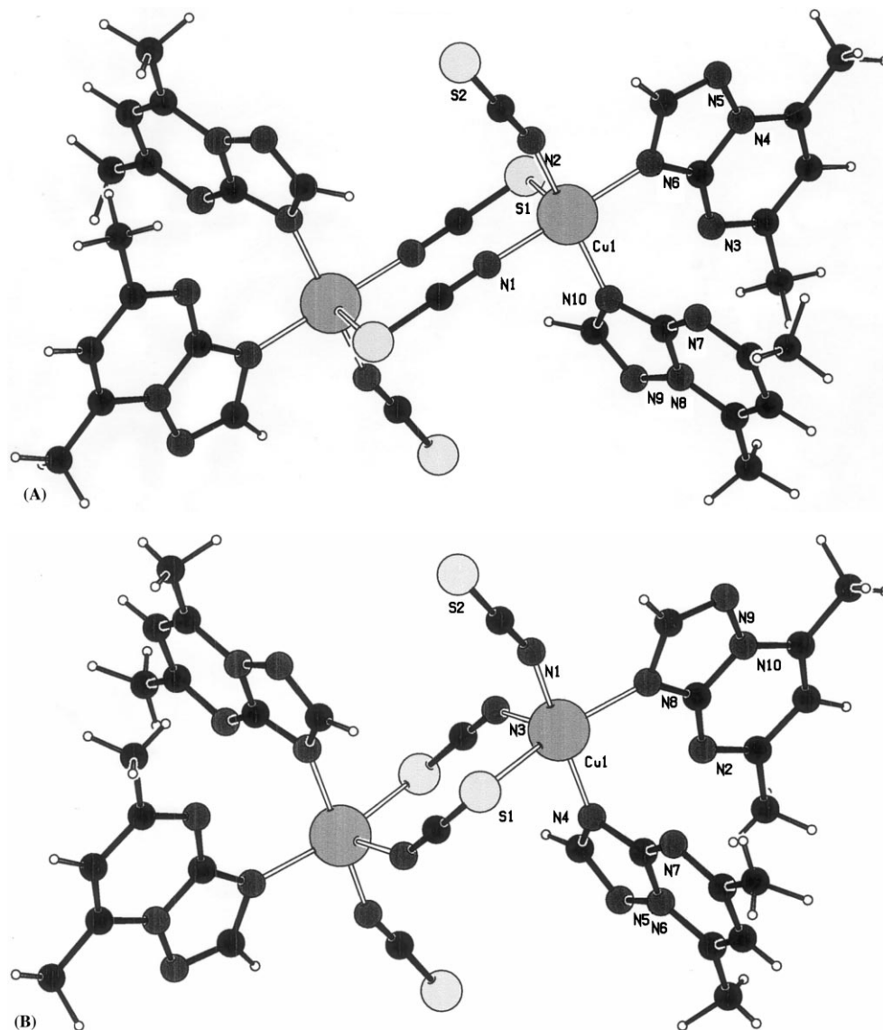
Fig. 29. Distortion isomerism in [\text{Cu}_2(\text{dmtp})_2(\text{NCS})_4] : (A) \alpha isomer with sulfur as apex; (B) \beta isomer with nitrogen as apex [190].
