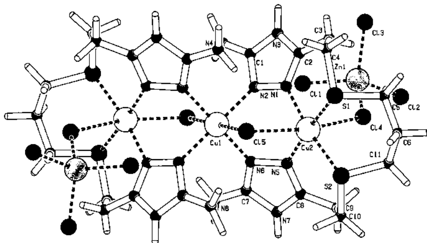
Fig. 17. Structure of the molecular unit of [\text{Cu}_3(\text{attn})_2\text{Cl}_2(\text{ZnCl}_4)_2] , \text{attn} = 1,9\text{-bis}(3\text{-aminotriazol-5-yl})\text{-}3,7\text{-dithianonane} [137].
