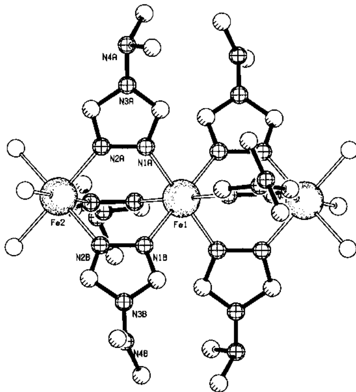
Fig. 7. Schematic representation of the trinuclear cation of [\text{Fe}(\text{Me}_2\text{Ntrz})_6(\text{H}_2\text{O})_6](\text{ClO}_4)_6 [107].
