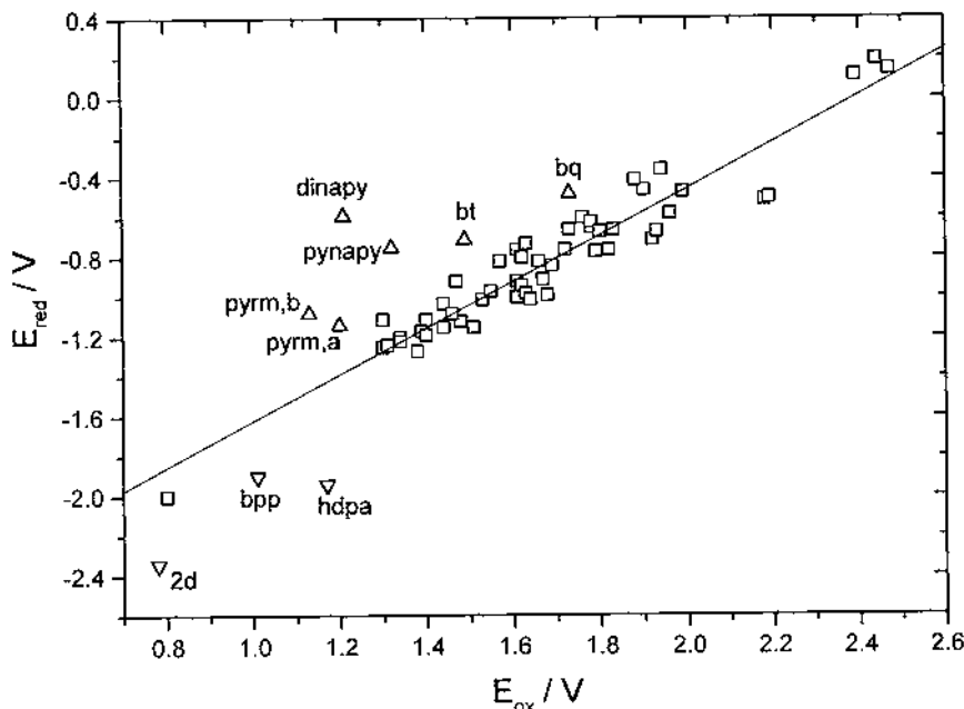
Fig. 1. A plot of reduction potentials E_{\text{red}} vs. oxidation potentials E_{\text{ox}} for a series of Ru(II) tris-polypyridyl complexes. Data against NHE taken from Ref. [24]. □ = well behaved points; Δ = deviating points, reversible processes; ▽ = reduction reported irreversible, only some representative points included. Abbreviations used: bt = 2,2'-bi-2-thiazoline; bq = 2,2'-biquinoline; dinapy = 5,6-dihydro-dipyrido[3,2-b:2',3'-j][1,10]phenanthroline; hdpa = di-2-pyridyl amine; pynapy = 2-(2-pyridyl)-1,8-naphthridine; bpp = 2,6-bis( N -pyrazolylpyridine), see Ref. [25]; 2d: see Ref. [26], pyrm,a and pyrm,b: see Ref. [27].
