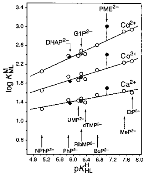
Fig. 2. Evidence for an enhanced stability of some M(PME) (●) complexes, based on the relationship between \log K_{ML}^M and pK_{HL}^H for the 1:1 complexes of Ca^{2+} , Co^{2+} , and Cd^{2+} with some simple phosphate monoester or phosphonate ligands: 4-nitrophenyl phosphate ( NPhP^{2-} ), phenyl phosphate ( PhP^{2-} ), uridine 5'-monophosphate ( UMP^{2-} ), D-ribose 5-monophosphate ( RibMP^{2-} ), thymidine [1-(2'-deoxy-β-D-ribofuranosyl)thymine] 5'-monophosphate ( dTMP^{2-} ), n -butyl phosphate ( BuP^{2-} ), methanephosphonate ( MeP^{2-} ), and ethanephosphonate ( EtP^{2-} ) (from left to right) (○). The least-squares lines are drawn through the corresponding eight data sets [49,50]; the equations for these base lines are given in Table 1 (entries 2, 6 and 10). The vertical broken lines emphasize the stability differences of the M(PME) (●) complexes to the corresponding reference lines; these differences are equal to \log \Delta_{M(PME)} (Eq. (10)), the values of which are listed in column 6 of Table 2. The equilibrium constants for the data points due to the PME systems are taken from Tables 1 and 8 of Ref. [49] (see also Table 2). For further comparison also the data points for the DHAP (◆) and G1P (⊗) systems, to be discussed in Section 4.1 (Table 4 [61]), are inserted into this figure. All plotted equilibrium constant values refer to aqueous solutions at 25°C and I = 0.1 M ( NaNO_3 ).
