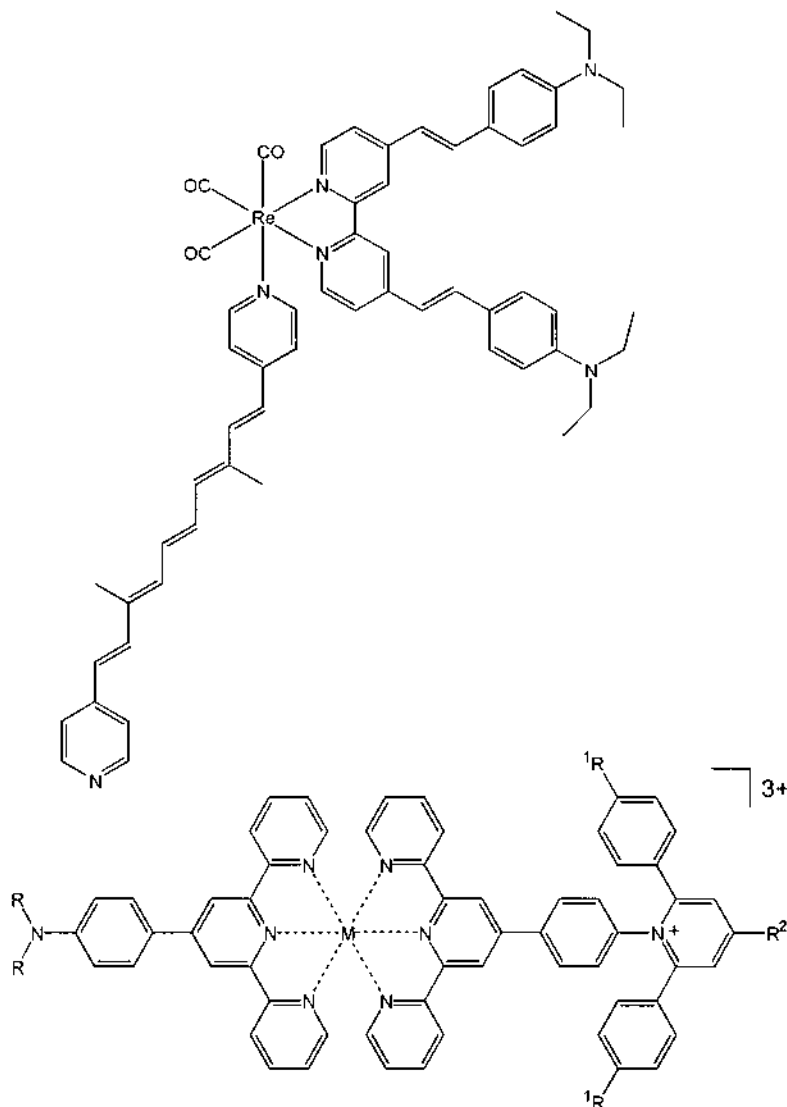
Fig. 6. Examples of complexes whose MLCT excitation leads to a long-lived charge separation. Top: [\text{Re}(\text{BPP})(\text{CO})_3(\text{DEAS-bpy})]^+ [85,86]. Bottom: [(\text{Me}_2\text{N-}p\text{-phenyl-trpy})\text{M}(p\text{-phenyl-triarylpyridinium-trpy})]^{3+} ; \text{M} = \text{Ru} or \text{Os} ; [87].
