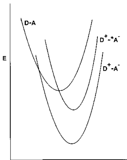
Fig. 11. Acceleration of an inverted electron transfer by formation of a low-lying excited state. Formation of the ground-state product \text{D}^+-\text{A}^- occurs in the Marcus inverted region with a considerable barrier. However, if the reduced acceptor (shown) or the oxidized donor possesses a low-lying excited state, the electron transfer can form this state with a lower or non-existent barrier (as shown). This phenomenon is responsible not only for the acceleration of an inverted electron transfer, but also for (electro)chemiluminescence [67] and for the absence of Marcus inverted behavior [44] in some highly energetic redox reactions.
