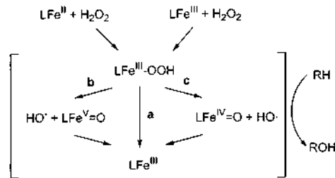
Fig. 14. Possible pathways for the [\text{Fe}(\text{bpmen})(\text{CH}_3\text{CN})_2]^{2+} catalyzed \text{H}_2\text{O}_2 alkane hydroxylation.
