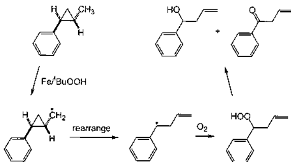
Fig. 8. Radical rearrangement on the [\text{Fe}_2\text{O}(\text{H}_2\text{O})_2(\text{tmima})_2]^{4+} catalyzed 'BuOOH oxidation of trans -2-phenylmethylcyclopropane.
