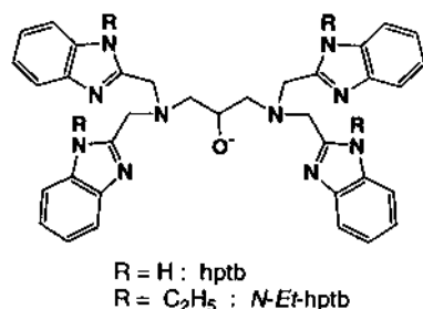
Fig. 4. Chemical structure of hptb and N-Et-hptb.
