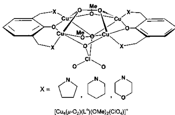
Fig. 12. Structure of [\text{Cu}_4(\mu\text{-O}_2)(\text{L}'')_2(\text{OMe})_2(\text{ClO}_4)]^+ (36).
