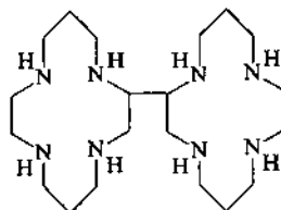
3 , 2,2'-bi(cyclam)
