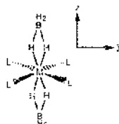
(\text{dmpe})_2\text{Ti}(\eta^2\text{-BH}_4)_2 [44,45]
