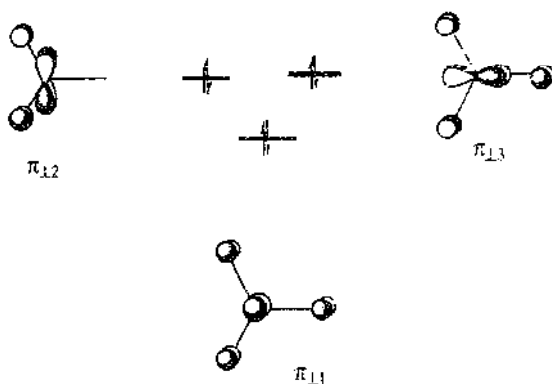
Fig. 3. \pi -type orbital interaction between metal atom ( \pi_{\perp 1}, \pi_{\perp 2}, \pi_{\perp 3} ) and ligands.
