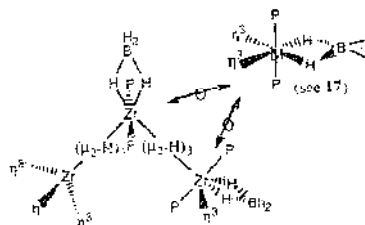
(\eta^2\text{-BH}_4)_2\text{Zr}(\mu_2\text{-H})_2\text{Zr}(\text{PMe}_3)_2(\eta^2\text{-BH}_4)(\mu_2\text{-H})_2\text{Zr}(\text{PMe}_3)_2(\eta^2\text{-BH}_4)(\eta^2\text{-BH}_4) [63]
