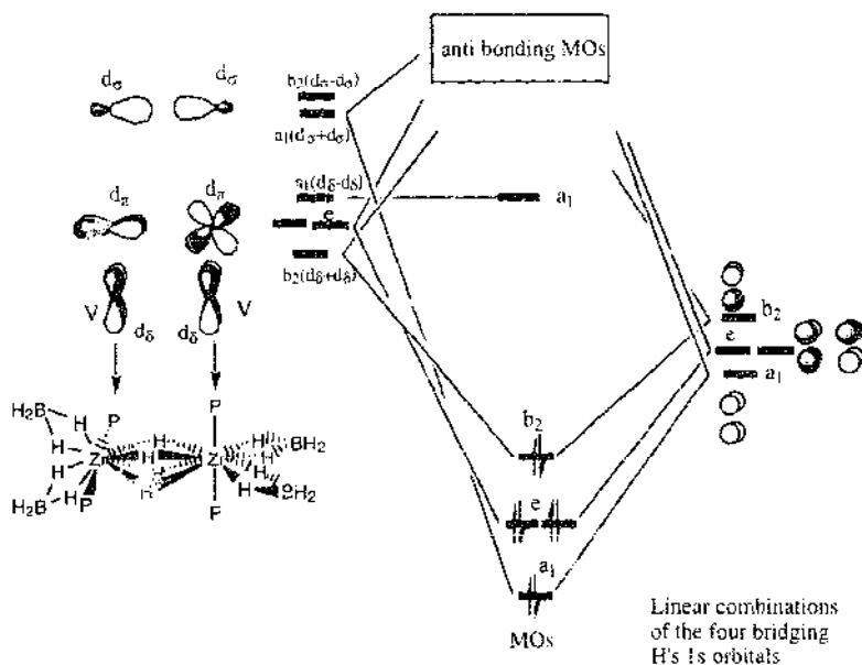
Fig. 9. The orbital interaction between four bridging hydrogen atoms and the (\text{PMe}_3)_2\text{Zr}(\eta^2\text{-BH}_4)_2(\mu_2\text{-H})_2 fragment in (\text{PMe}_3)_2\text{Zr}(\eta^2\text{-BH}_4)_2(\mu_2\text{-H})_2 . (Orbital symmetries are assigned based on a pseudo- D_{2h} point group.)
