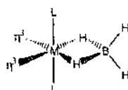
(\text{thf})_3\text{Sc}(\eta^1\text{-BH}_4)_2(\eta^3\text{-BH}_4) [38]
