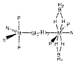
(\text{pmp})(\eta^2\text{-BH}_4)(\text{H})(\mu_2\text{-H})_2\text{H}(\text{pmp})(\eta^2\text{-BH}_4)_2 [65]
