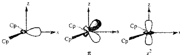
Fig. 7. The frontier orbitals of a \text{Cp}_2\text{M} fragment.
