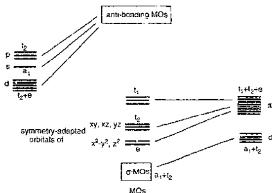
Fig. 5. Orbital interaction diagram for a tetrahedral M(\eta^3\text{-BH}_3)_2\text{L}_2 complex.
