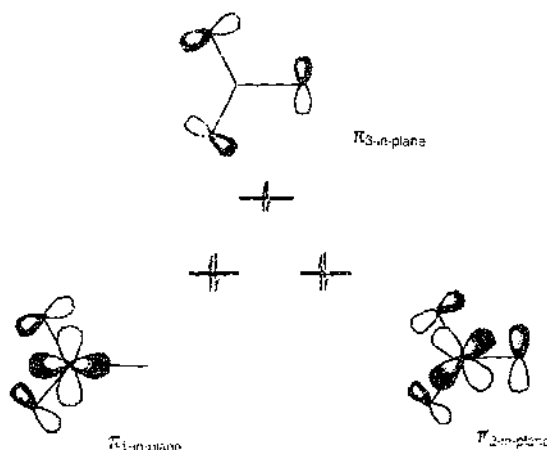
Fig. 4. \pi_{3\text{-in-plane}} -type orbital interaction between metal atom ( x^2 , y^2 , xy ) and ligands.
