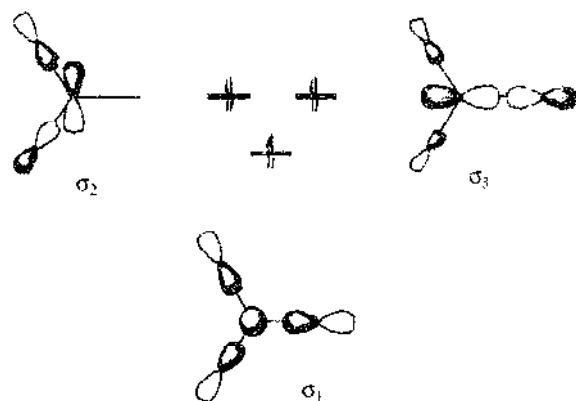
Fig. 2. \sigma -type orbital interaction between metal atoms ( \sigma_1, \sigma_2, \sigma_3 ) and ligands.
