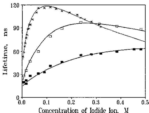
Fig. 5. Influence of ionic strength on luminescence lifetime vs. iodide ion concentration in aqueous solution of dicyanocuprate at ambient temperature, \lambda_{exc} = 266 nm; \mu = 0.5 M (■); \mu = 2.5 M (□); \mu = 5.0 M (*) [17].
