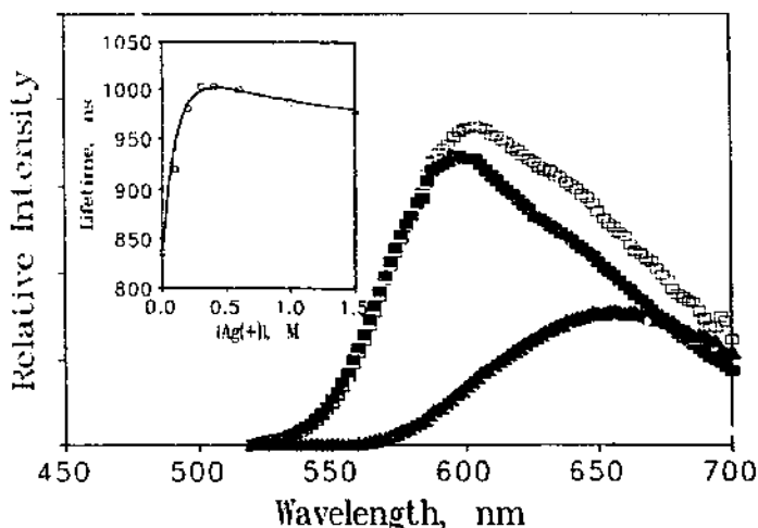
Fig. 2. The calculated luminescence spectra of ^*[Ru(phen)_3]Ag_n^{n+2+} species; (■) n=0 , (□) n=1 and (▲) n=2 . The inset shows the change in luminescence lifetime with silver ion concentration in aqueous solution of [Ru(phen)_3]^{2+} at 3 M ionic strength and ambient temperature; measured (□) and calculated values (---).
