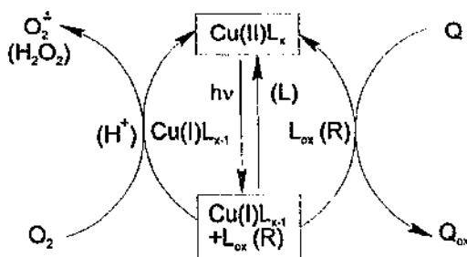
Fig. 1. Environmentally interesting photo-oxidations based on Cu(II)–Cu(I) photocatalytic redox cycle in the Cu(II)/Cu(I)–L(Q)– \text{O}_2 homogeneous system ( \text{L} and/or \text{Q} =pollutant, \text{R} = \text{L}_{\text{ox}} or \text{R} \neq \text{L}_{\text{ox}} =oxidant).
