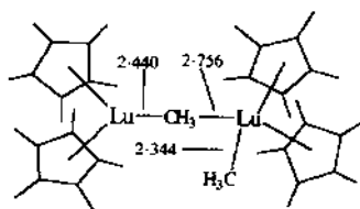
Fig. 23. The structure of [\text{Cp}_2^*\text{Lu}(\mu\text{-Me})\text{LuCp}_2^*(\text{Me})] .
