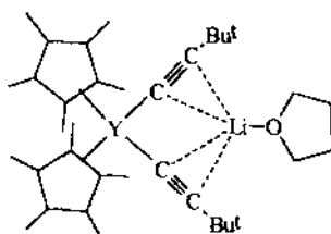
Fig. 21. The structure of [\text{Cp}_2^*\text{Y}(\mu\text{-C}\equiv\text{CBu}^t)_2\text{Li}(\text{THF})] .
