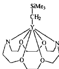
Fig. 10. The structure of [Ln(DAC)CH 2 SiMe 3 ].
