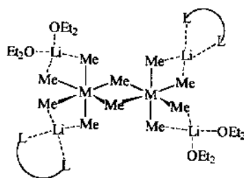
Fig. 8. The structure of [\{Li_2(teed)(Et_2O)_2\}_2Lu_2(CH_3)_{10}] .
