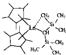
Fig. 22. The structure of [\text{Cp}_2^*\text{Ln}\{\text{CH}(\text{SiMe}_3)_2\}] .
