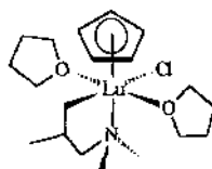
Fig. 28. The structure of [(\text{C}_5\text{H}_5)\text{Lu}(\text{CH}_2\text{CH}(\text{Me})\text{CH}_2\text{NMe}_2)\text{Cl}(\text{THF})_2] .
