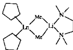
Fig. 20. The structure of [Cp 2 Ln(μ-Me) 2 Li(tmed)].
