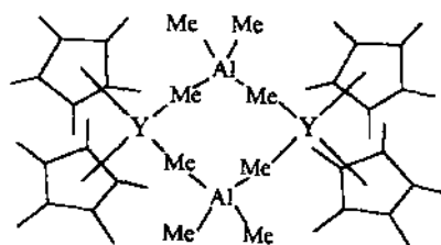
Fig. 24. The structure of [\text{Cp}^*_2\text{Y}(\mu\text{-Me}_2\text{AlMe}_2)_2\text{YCp}^*_2] .
