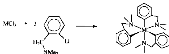
Fig. 12. The structure of [M(\text{o-C}_6\text{H}_4\text{CH}_2\text{NMe}_2)_3] ( M = \text{Er, Yb, Lu} ).
